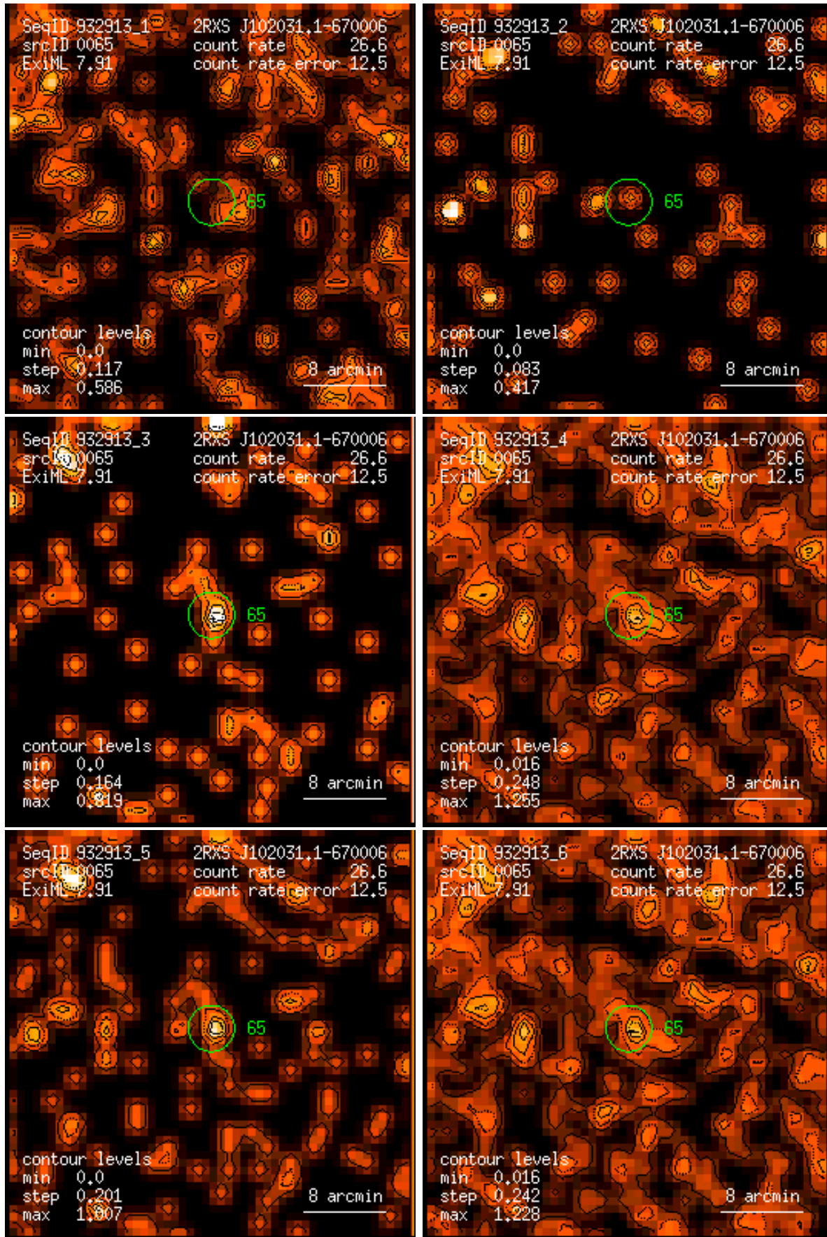
Figure 65: RASS 932913: detection 0065: band rate images, Gaussian filter: (1) PSPC channels 11 – 41, (2) 52 – 90, (3) 91 – 201, (4) 11 – 235, (5) 52 – 201, (6) 11 – 201. Broad band rates in counts/ks. Band rate contour levels in counts/ks/arcmin 2 .
