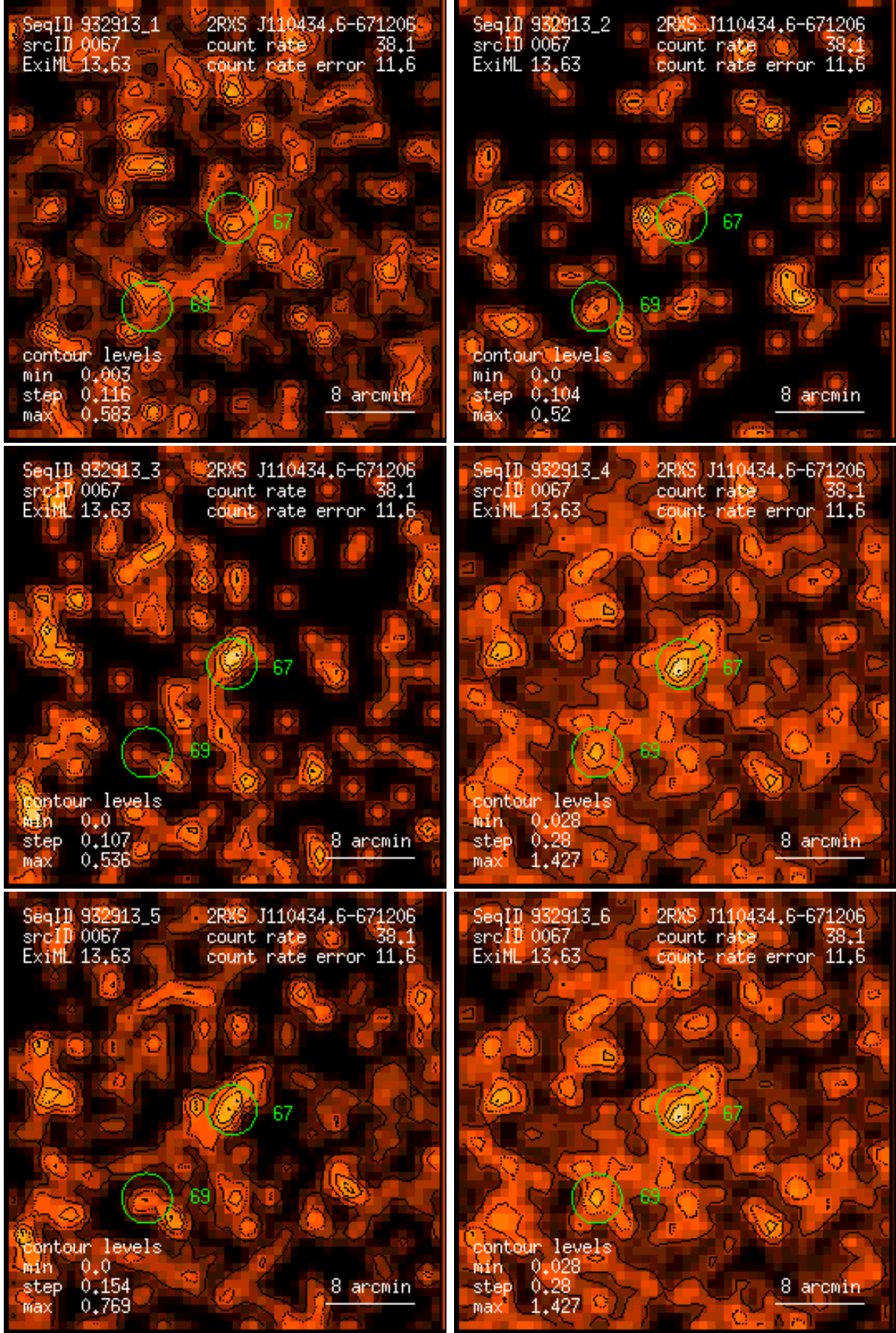
Figure 67: RASS 932913: detection 0067: band rate images, Gaussian filter: (1) PSPC channels 11 – 41, (2) 52 – 90, (3) 91 – 201, (4) 11 – 235, (5) 52 – 201, (6) 11 – 201. Broad band rates in counts/ks. Band rate contour levels in counts/ks/arcmin 2 .
