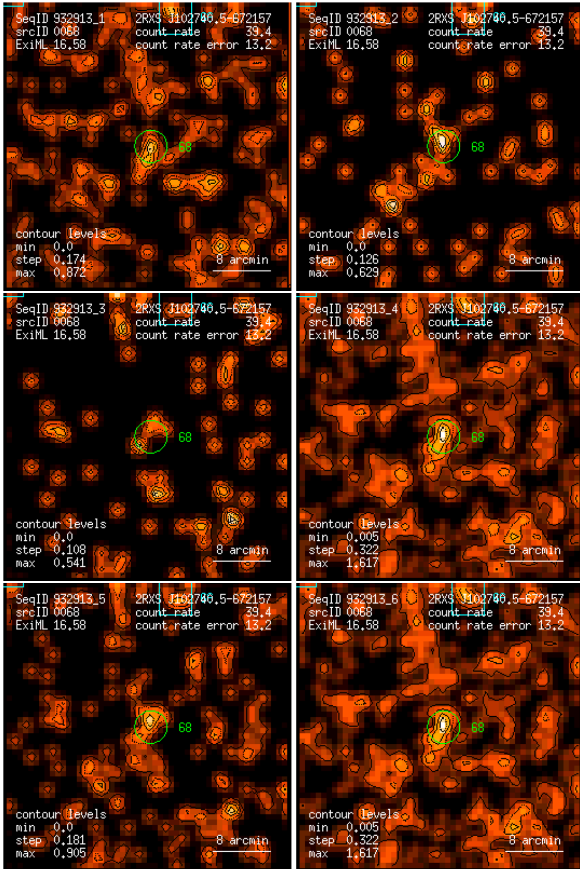
Figure 68: RASS 932913: detection 0068: band rate images, Gaussian filter: (1) PSPC channels 11 – 41, (2) 52 – 90, (3) 91 – 201, (4) 11 – 235, (5) 52 – 201, (6) 11 – 201. Broad band rates in counts/ks. Band rate contour levels in counts/ks/arcmin 2 .
