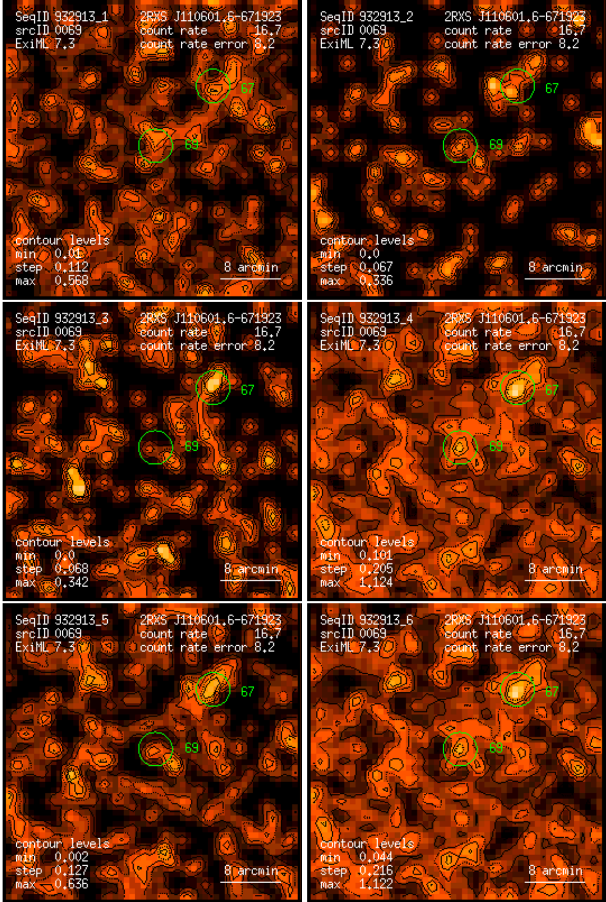
Figure 69: RASS 932913: detection 0069: band rate images, Gaussian filter: (1) PSPC channels 11 – 41, (2) 52 – 90, (3) 91 – 201, (4) 11 – 235, (5) 52 – 201, (6) 11 – 201. Broad band rates in counts/ks. Band rate contour levels in counts/ks/arcmin 2 .
