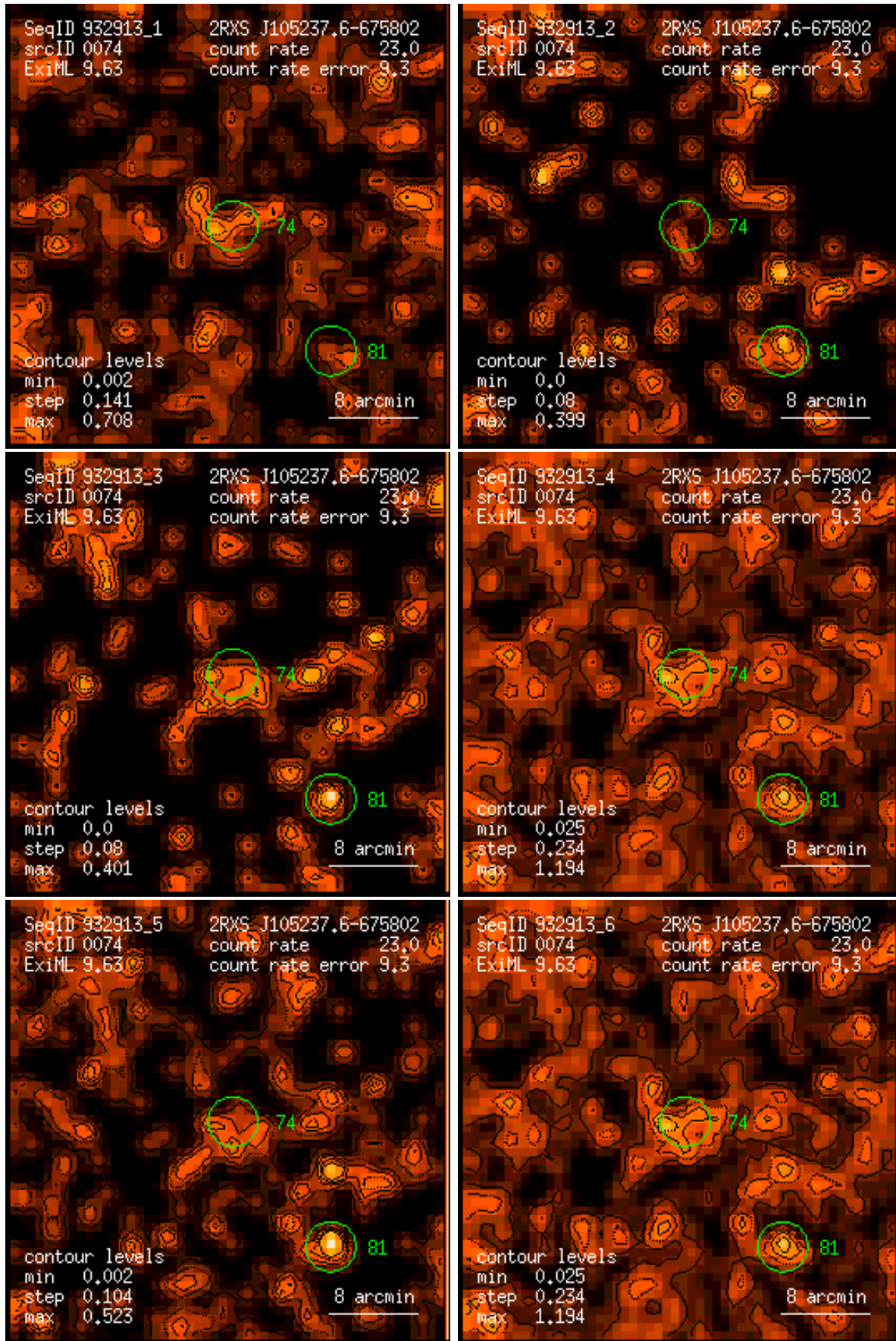
Figure 74: RASS 932913: detection 0074: band rate images, Gaussian filter: (1) PSPC channels 11 – 41, (2) 52 – 90, (3) 91 – 201, (4) 11 – 235, (5) 52 – 201, (6) 11 – 201. Broad band rates in counts/ks. Band rate contour levels in counts/ks/arcmin 2 .
