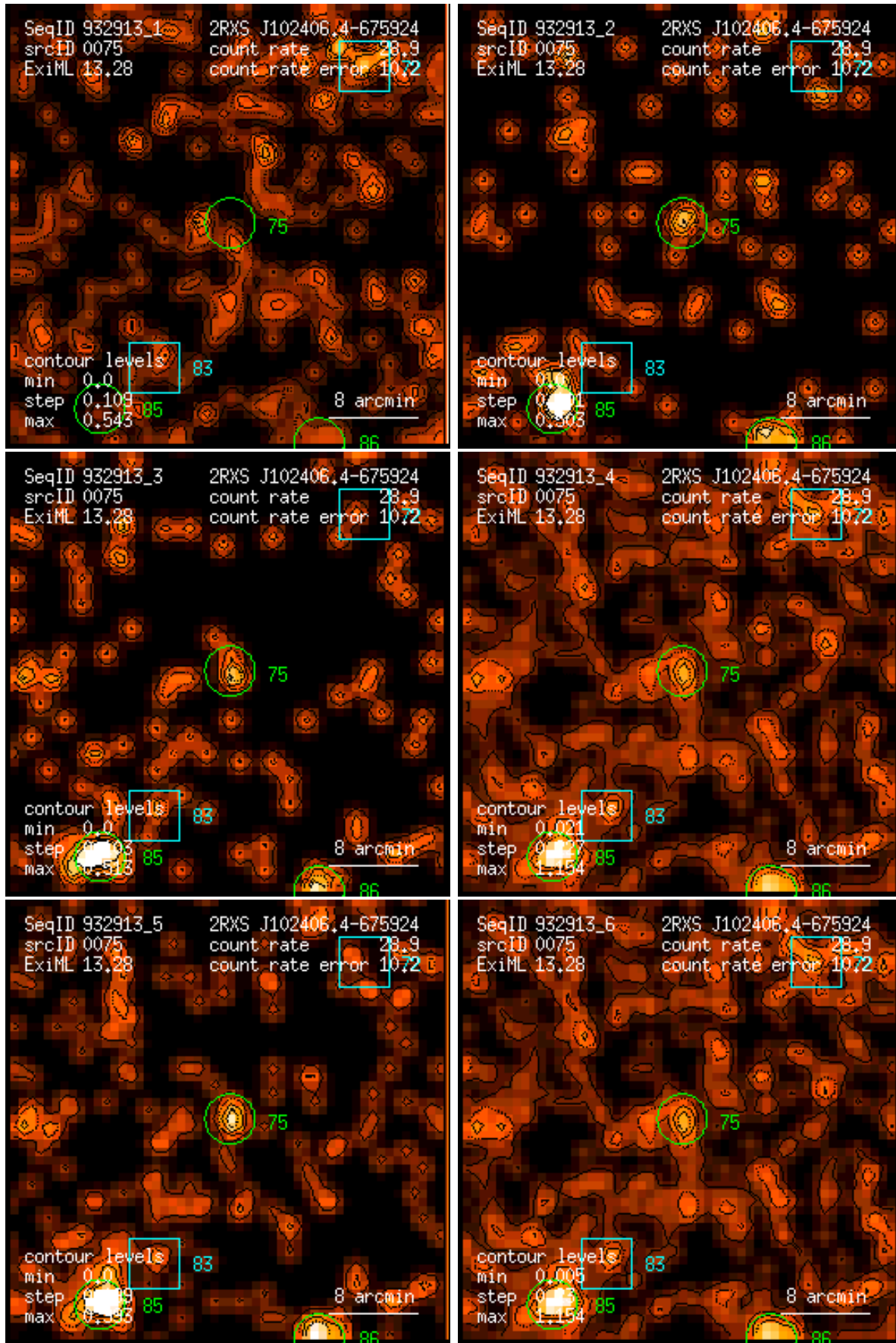
Figure 75: RASS 932913: detection 0075: band rate images, Gaussian filter: (1) PSPC channels 11 – 41, (2) 52 – 90, (3) 91 – 201, (4) 11 – 235, (5) 52 – 201, (6) 11 – 201. Broad band rates in counts/ks. Band rate contour levels in counts/ks/arcmin 2 .
