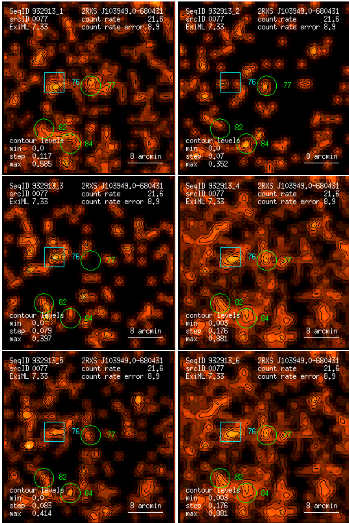
Figure 77: RASS 932913: detection 0077: band rate images, Gaussian filter: (1) PSPC channels 11 – 41, (2) 52 – 90, (3) 91 – 201, (4) 11 – 235, (5) 52 – 201, (6) 11 – 201. Broad band rates in counts/ks. Band rate contour levels in counts/ks/arcmin 2 .
