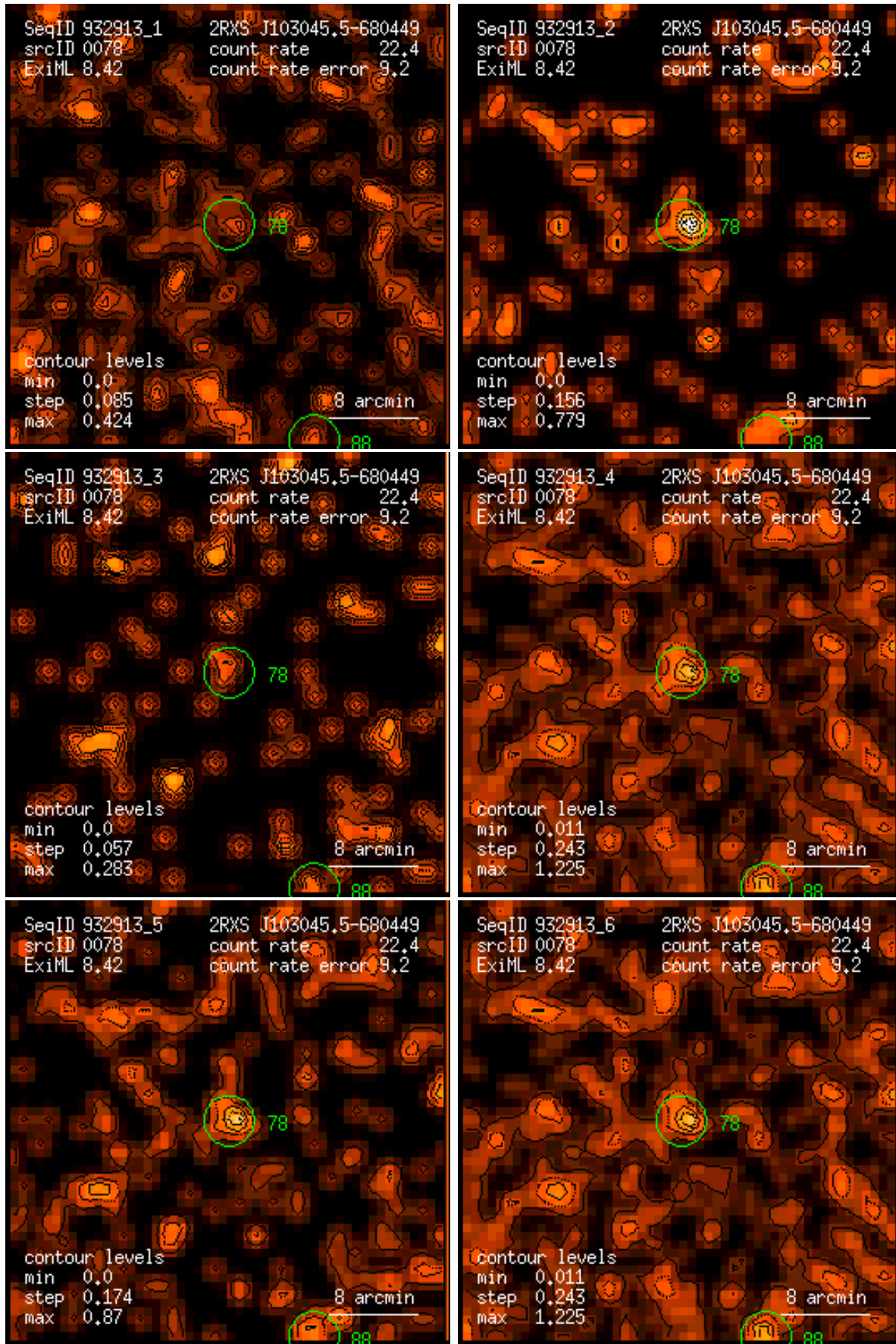
Figure 78: RASS 932913: detection 0078: band rate images, Gaussian filter: (1) PSPC channels 11 – 41, (2) 52 – 90, (3) 91 – 201, (4) 11 – 235, (5) 52 – 201, (6) 11 – 201. Broad band rates in counts/ks. Band rate contour levels in counts/ks/arcmin 2 .
