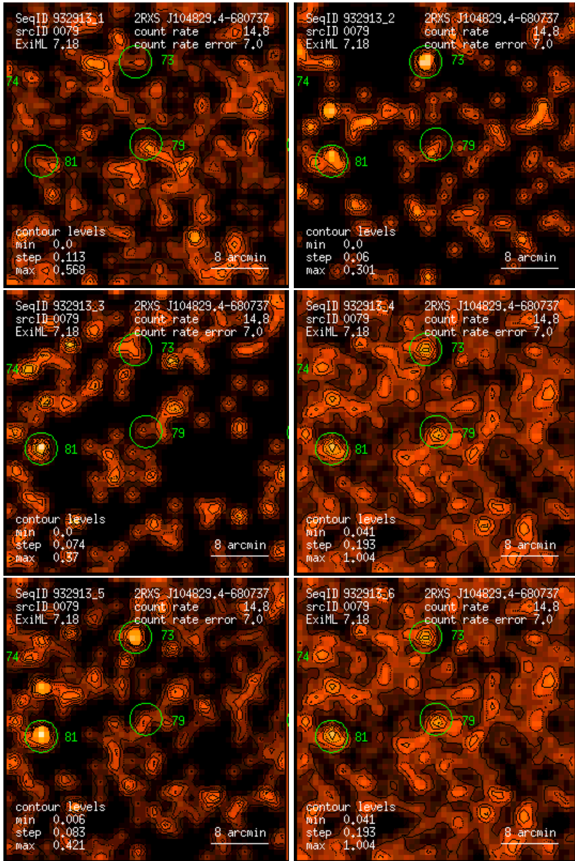
Figure 79: RASS 932913: detection 0079: band rate images, Gaussian filter: (1) PSPC channels 11 – 41, (2) 52 – 90, (3) 91 – 201, (4) 11 – 235, (5) 52 – 201, (6) 11 – 201. Broad band rates in counts/ks. Band rate contour levels in counts/ks/arcmin 2 .
