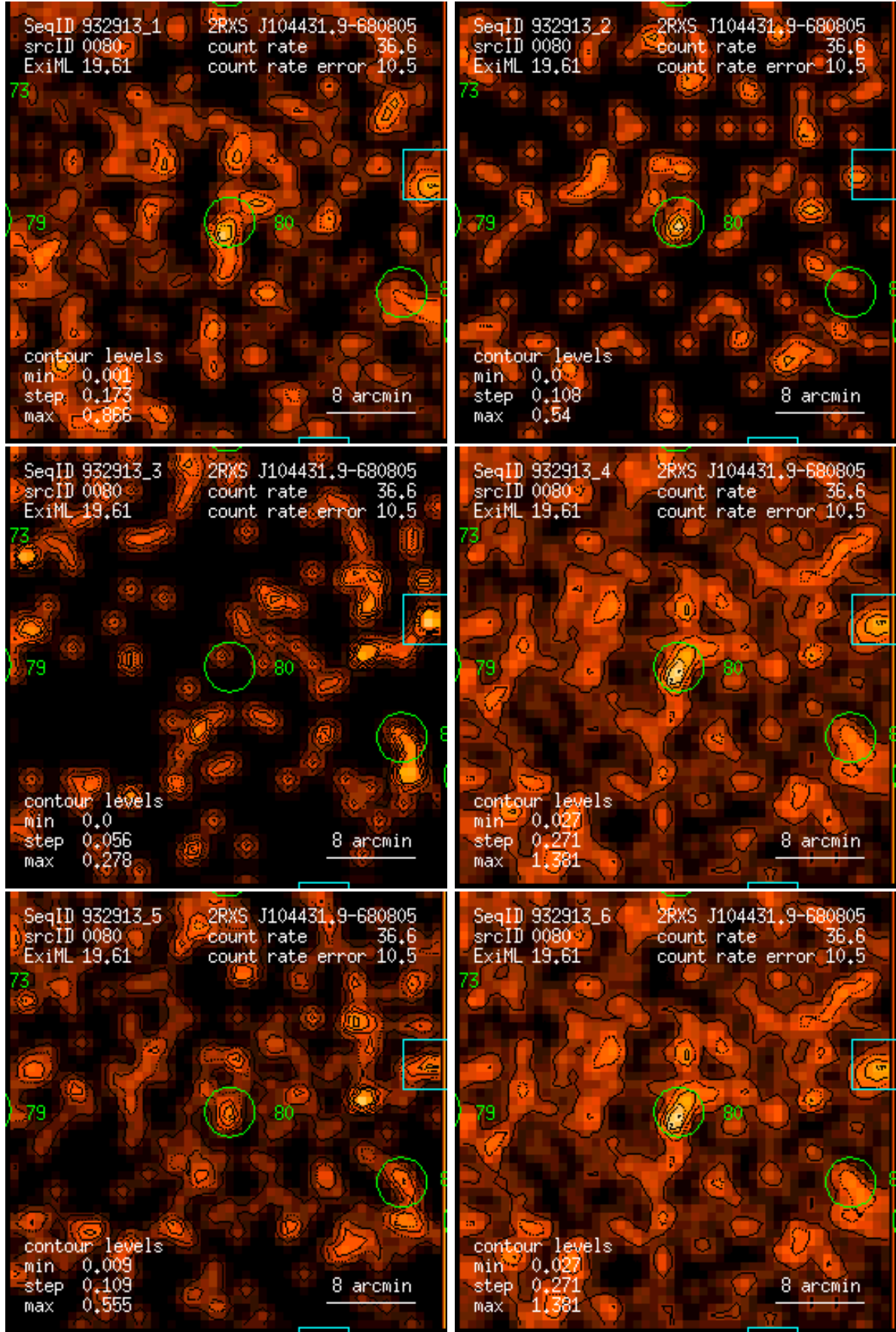
Figure 80: RASS 932913: detection 0080: band rate images, Gaussian filter: (1) PSPC channels 11 – 41, (2) 52 – 90, (3) 91 – 201, (4) 11 – 235, (5) 52 – 201, (6) 11 – 201. Broad band rates in counts/ks. Band rate contour levels in counts/ks/arcmin 2 .
