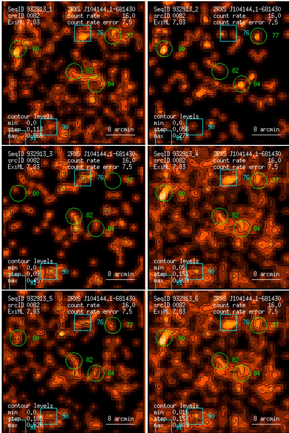
Figure 82: RASS 932913: detection 0082: band rate images, Gaussian filter: (1) PSPC channels 11 – 41, (2) 52 – 90, (3) 91 – 201, (4) 11 – 235, (5) 52 – 201, (6) 11 – 201. Broad band rates in counts/ks. Band rate contour levels in counts/ks/arcmin 2 .
