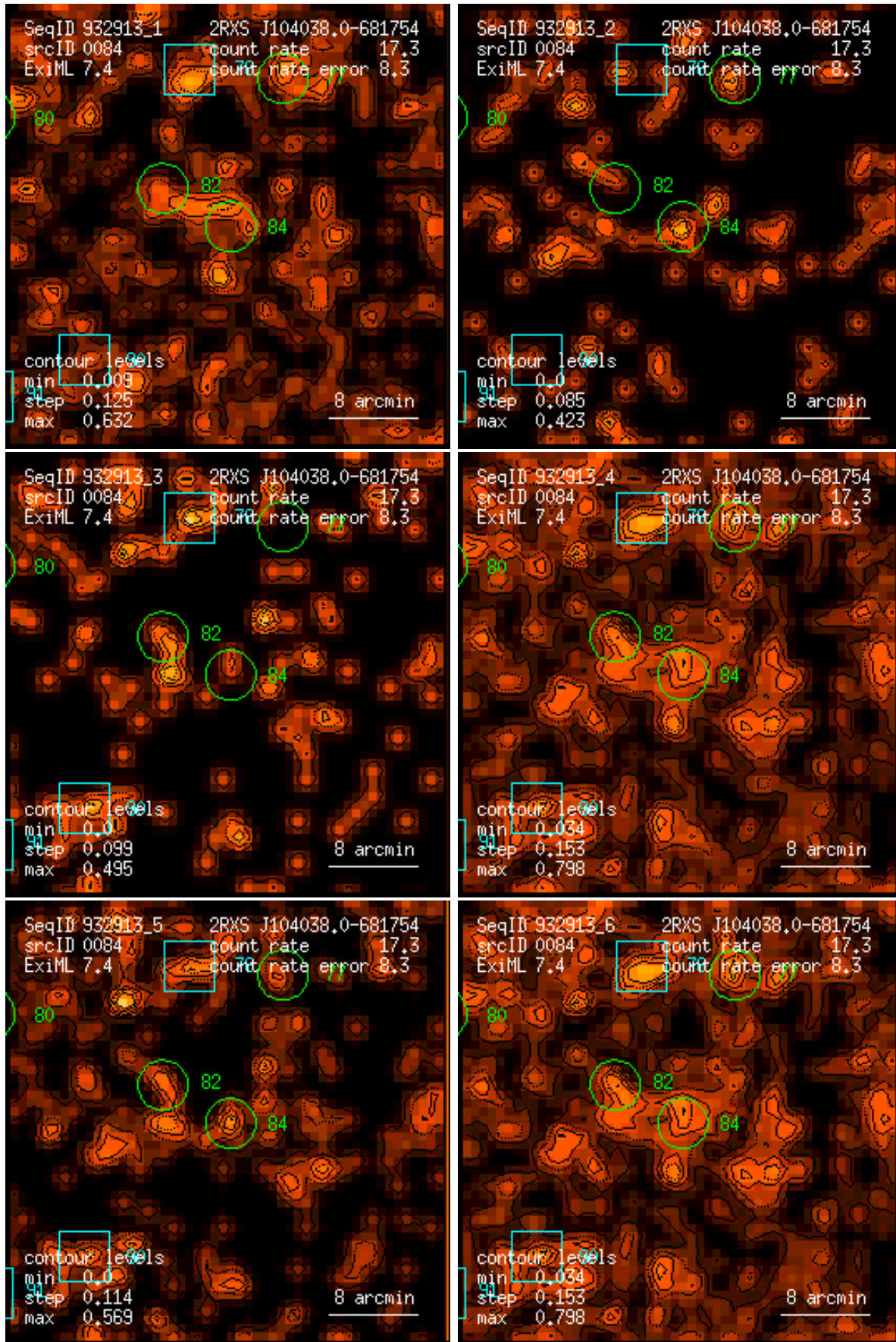
Figure 84: RASS 932913: detection 0084: band rate images, Gaussian filter: (1) PSPC channels 11 – 41, (2) 52 – 90, (3) 91 – 201, (4) 11 – 235, (5) 52 – 201, (6) 11 – 201. Broad band rates in counts/ks. Band rate contour levels in counts/ks/arcmin 2 .
