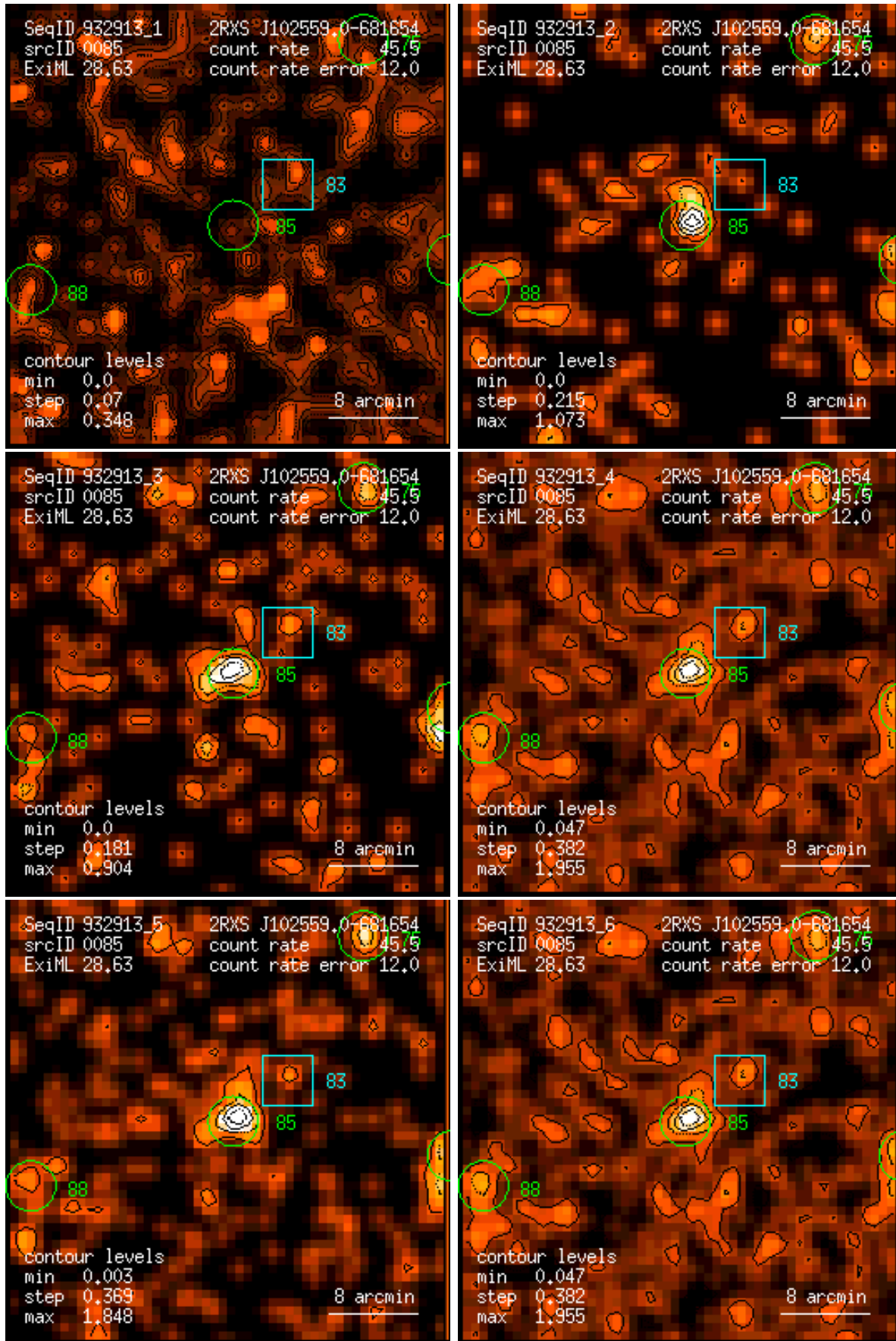
Figure 85: RASS 932913: detection 0085: band rate images, Gaussian filter: (1) PSPC channels 11 – 41, (2) 52 – 90, (3) 91 – 201, (4) 11 – 235, (5) 52 – 201, (6) 11 – 201. Broad band rates in counts/ks. Band rate contour levels in counts/ks/arcmin 2 .
