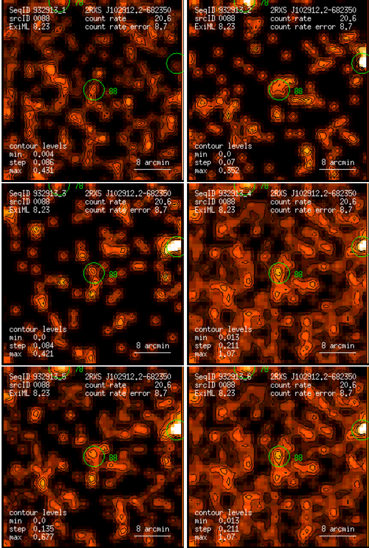
Figure 88: RASS 932913: detection 0088: band rate images, Gaussian filter: (1) PSPC channels 11 – 41, (2) 52 – 90, (3) 91 – 201, (4) 11 – 235, (5) 52 – 201, (6) 11 – 201. Broad band rates in counts/ks. Band rate contour levels in counts/ks/arcmin 2 .
