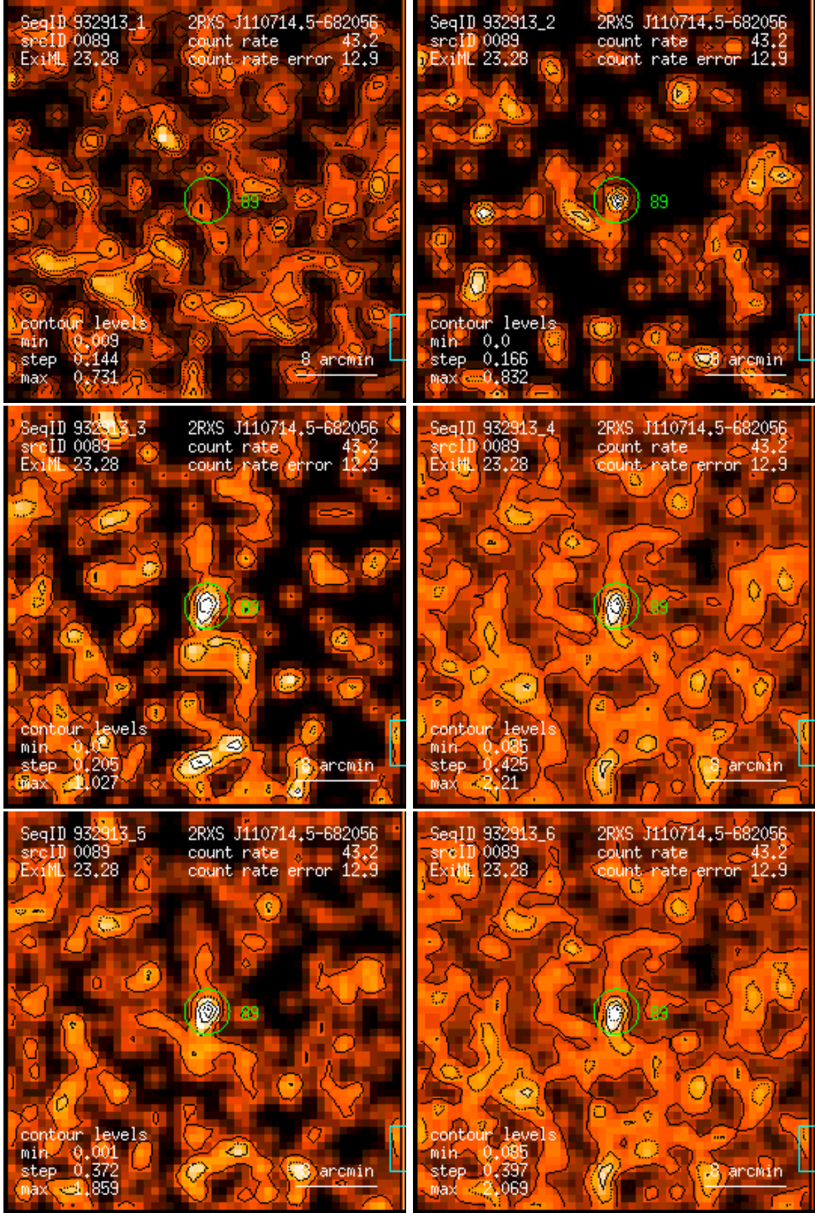
Figure 89: RASS 932913: detection 0089: band rate images, Gaussian filter: (1) PSPC channels 11 – 41, (2) 52 – 90, (3) 91 – 201, (4) 11 – 235, (5) 52 – 201, (6) 11 – 201. Broad band rates in counts/ks. Band rate contour levels in counts/ks/arcmin 2 .
