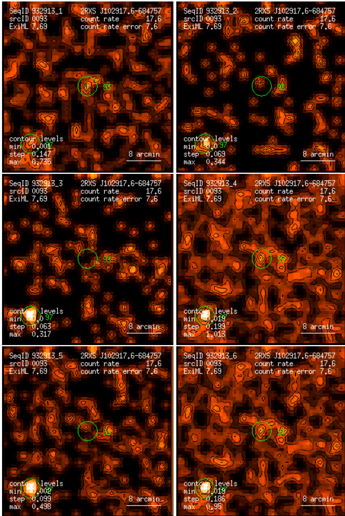
Figure 93: RASS 932913: detection 0093: band rate images, Gaussian filter: (1) PSPC channels 11 – 41, (2) 52 – 90, (3) 91 – 201, (4) 11 – 235, (5) 52 – 201, (6) 11 – 201. Broad band rates in counts/ks. Band rate contour levels in counts/ks/arcmin 2 .
