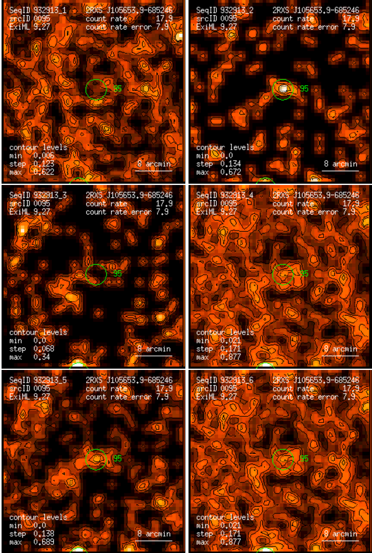
Figure 95: RASS 932913: detection 0095: band rate images, Gaussian filter: (1) PSPC channels 11 – 41, (2) 52 – 90, (3) 91 – 201, (4) 11 – 235, (5) 52 – 201, (6) 11 – 201. Broad band rates in counts/ks. Band rate contour levels in counts/ks/arcmin 2 .
