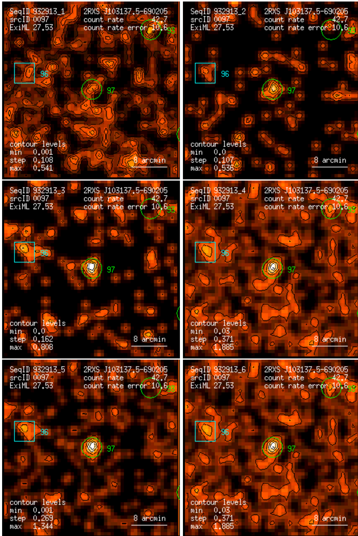
Figure 97: RASS 932913: detection 0097: band rate images, Gaussian filter: (1) PSPC channels 11 – 41, (2) 52 – 90, (3) 91 – 201, (4) 11 – 235, (5) 52 – 201, (6) 11 – 201. Broad band rates in counts/ks. Band rate contour levels in counts/ks/arcmin 2 .
