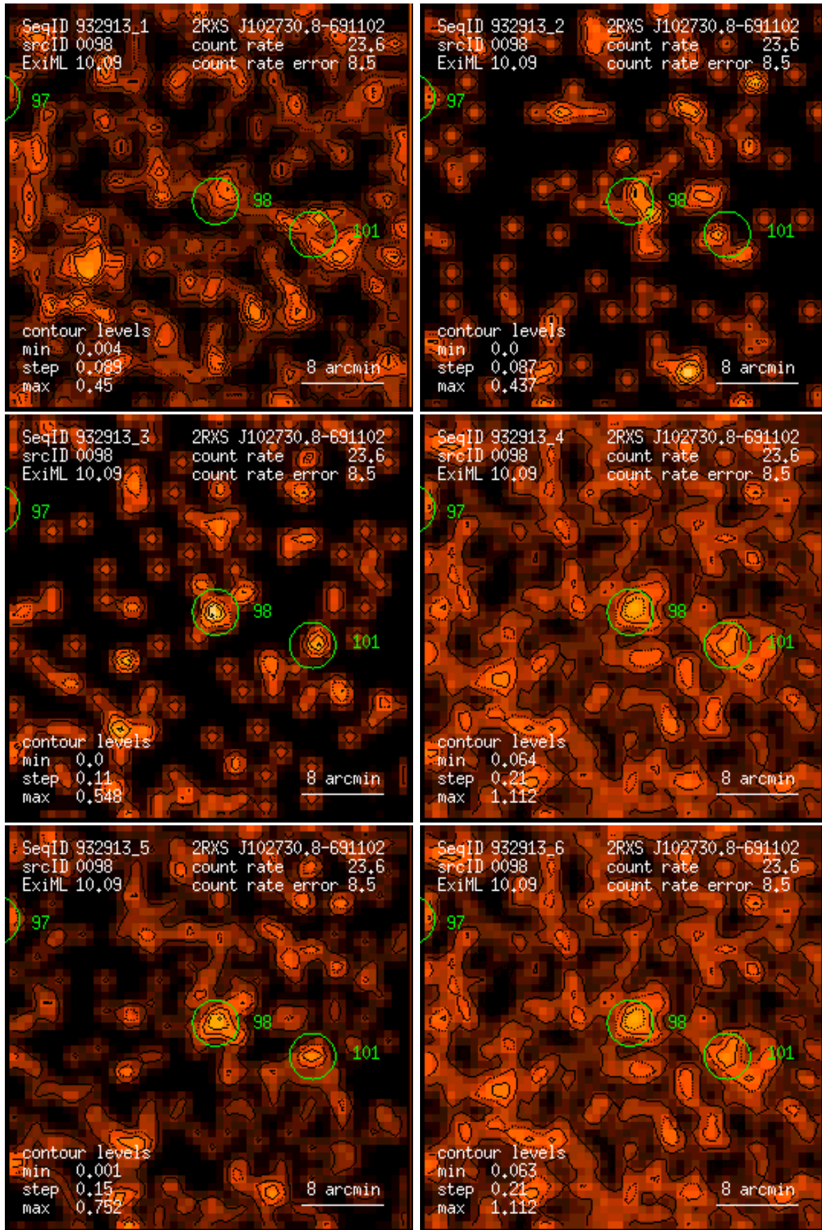
Figure 98: RASS 932913: detection 0098: band rate images, Gaussian filter: (1) PSPC channels 11 – 41, (2) 52 – 90, (3) 91 – 201, (4) 11 – 235, (5) 52 – 201, (6) 11 – 201. Broad band rates in counts/ks. Band rate contour levels in counts/ks/arcmin 2 .
