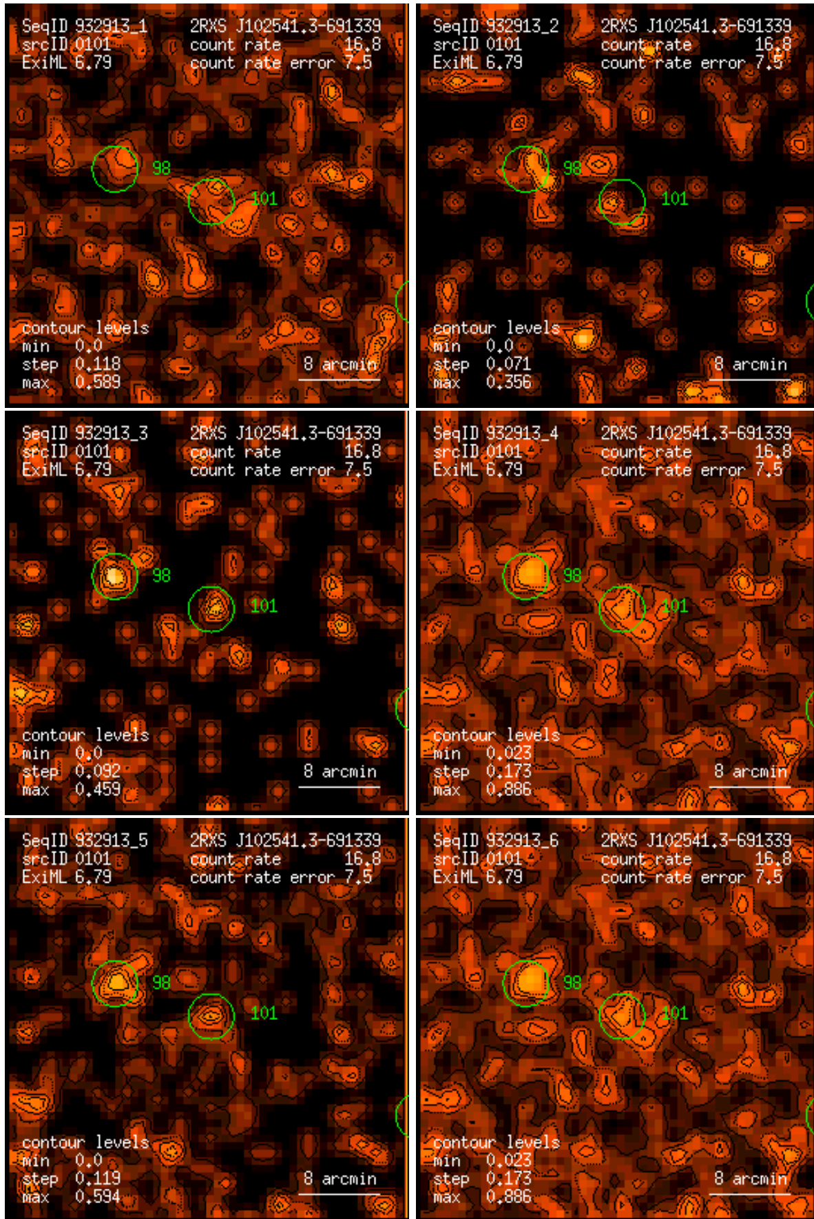
Figure 101: RASS 932913: detection 0101: band rate images, Gaussian filter: (1) PSPC channels 11 – 41, (2) 52 – 90, (3) 91 – 201, (4) 11 – 235, (5) 52 – 201, (6) 11 – 201. Broad band rates in counts/ks. Band rate contour levels in counts/ks/arcmin 2 .
