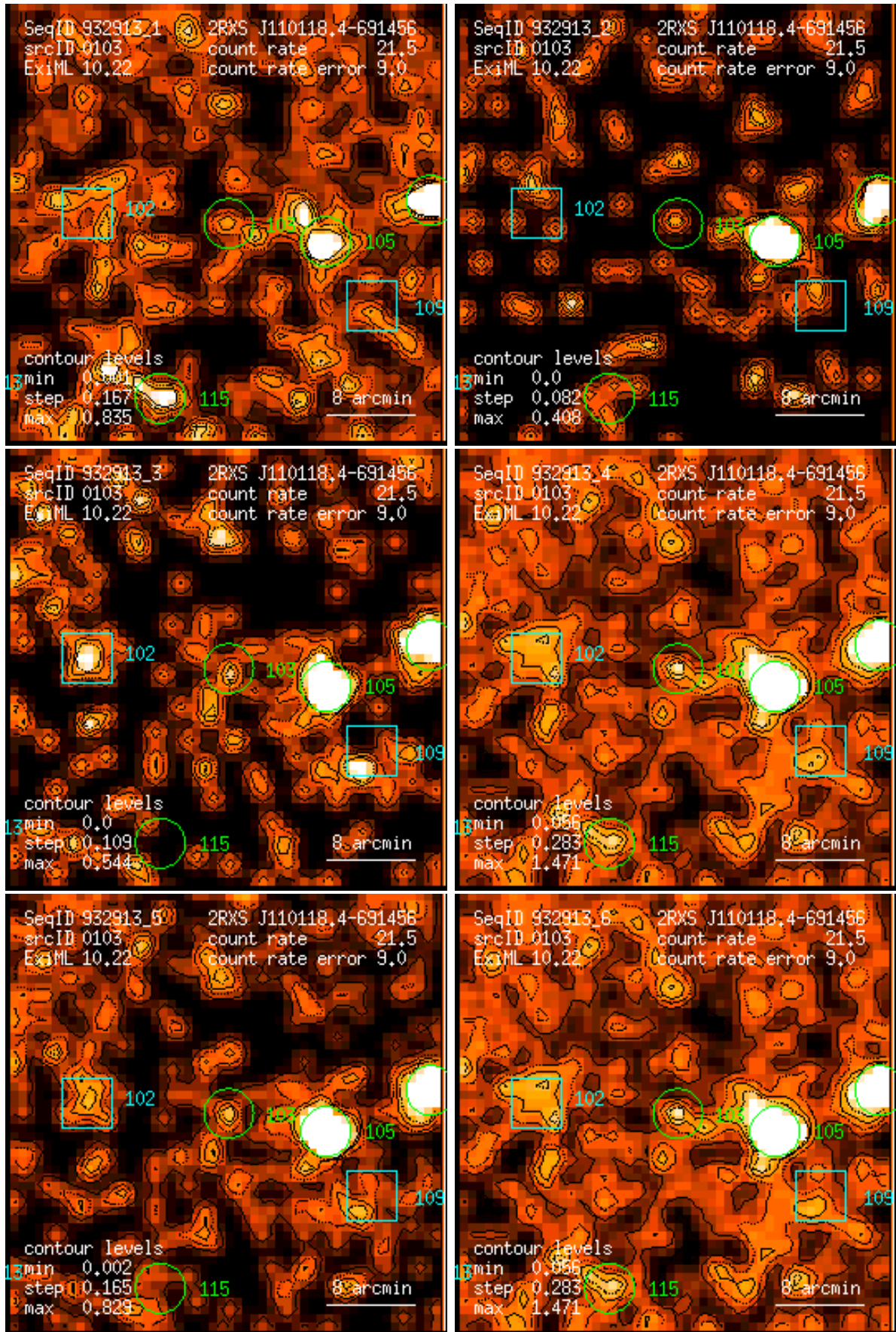
Figure 103: RASS 932913: detection 0103: band rate images, Gaussian filter: (1) PSPC channels 11 – 41, (2) 52 – 90, (3) 91 – 201, (4) 11 – 235, (5) 52 – 201, (6) 11 – 201. Broad band rates in counts/ks. Band rate contour levels in counts/ks/arcmin 2 .
