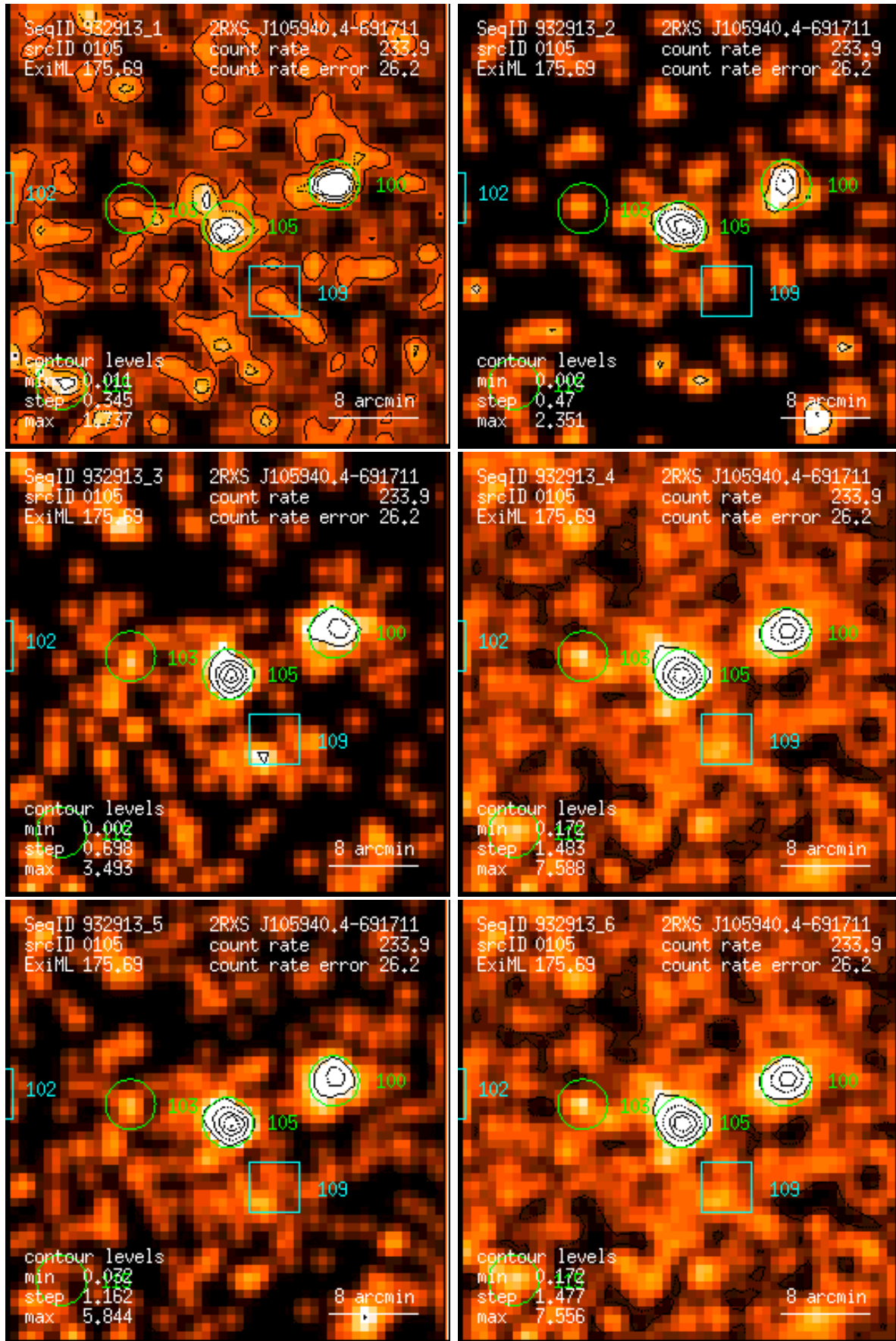
Figure 105: RASS 932913: detection 0105: band rate images, Gaussian filter: (1) PSPC channels 11 – 41, (2) 52 – 90, (3) 91 – 201, (4) 11 – 235, (5) 52 – 201, (6) 11 – 201. Broad band rates in counts/ks. Band rate contour levels in counts/ks/arcmin 2 .
