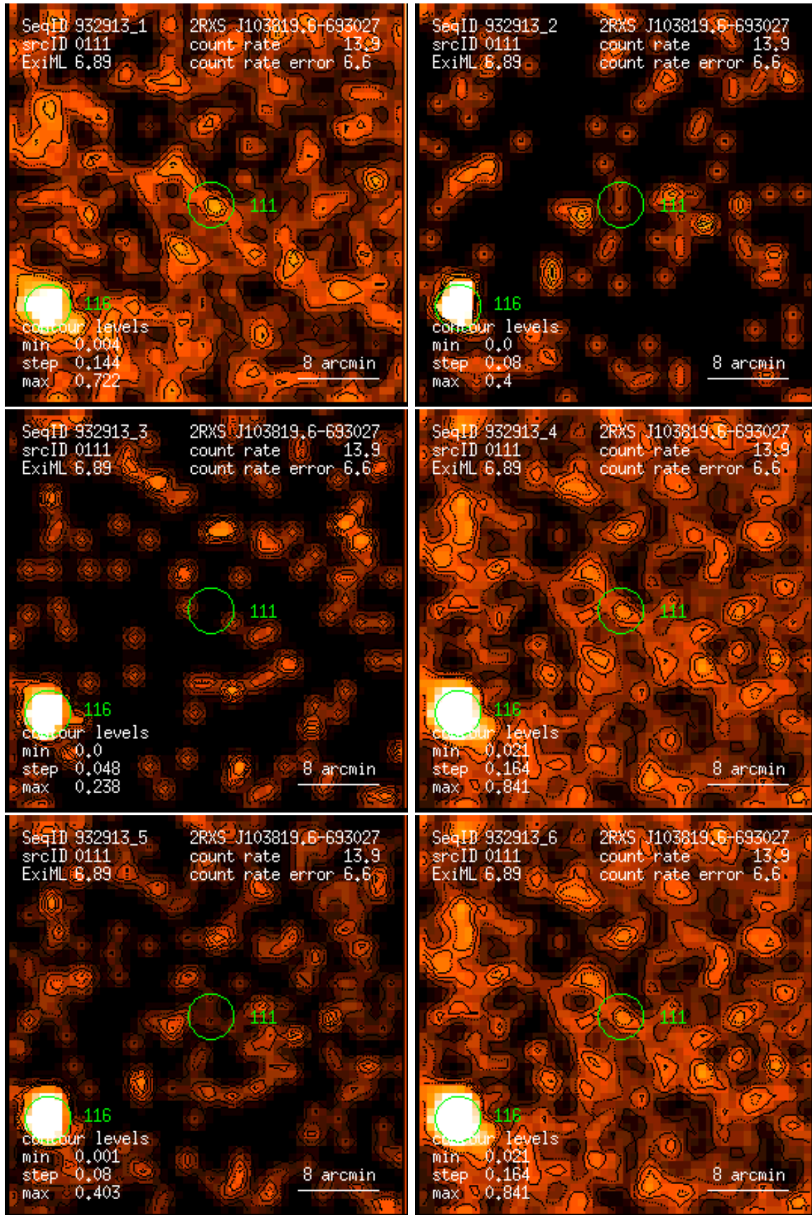
Figure 111: RASS 932913: detection 0111: band rate images, Gaussian filter: (1) PSPC channels 11 – 41, (2) 52 – 90, (3) 91 – 201, (4) 11 – 235, (5) 52 – 201, (6) 11 – 201. Broad band rates in counts/ks. Band rate contour levels in counts/ks/arcmin 2 .
