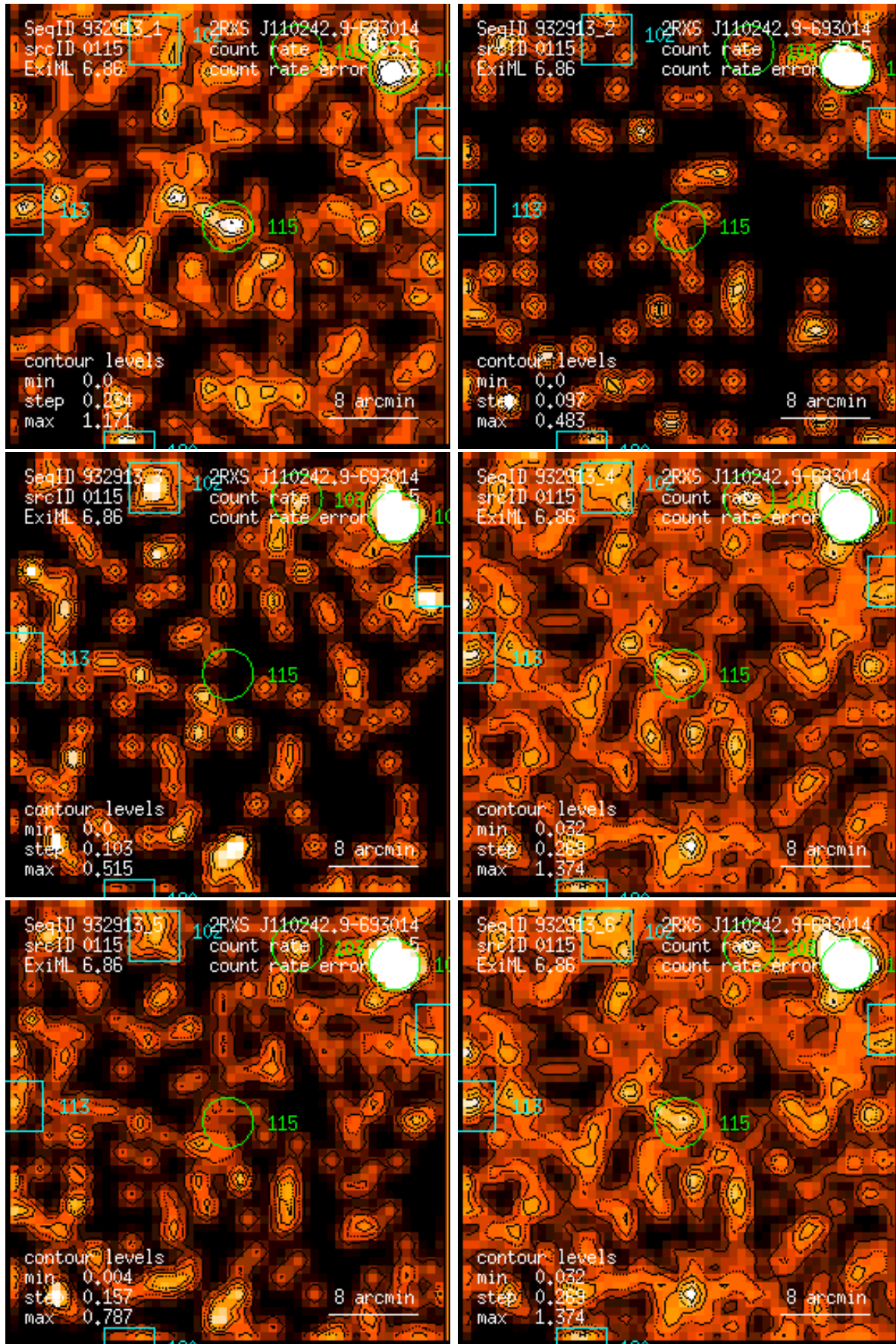
Figure 115: RASS 932913: detection 0115: band rate images, Gaussian filter: (1) PSPC channels 11 – 41, (2) 52 – 90, (3) 91 – 201, (4) 11 – 235, (5) 52 – 201, (6) 11 – 201. Broad band rates in counts/ks. Band rate contour levels in counts/ks/arcmin 2 .
