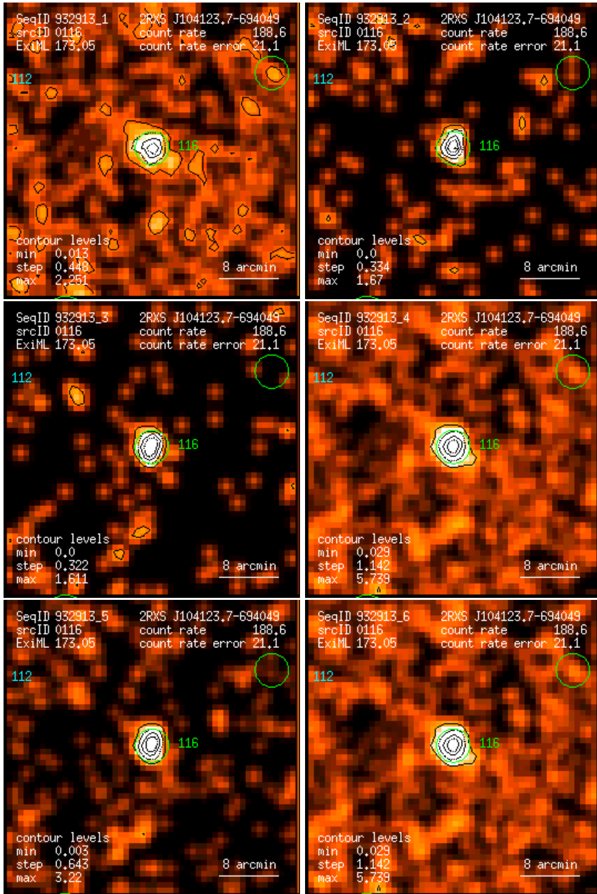
Figure 116: RASS 932913: detection 0116: band rate images, Gaussian filter: (1) PSPC channels 11 – 41, (2) 52 – 90, (3) 91 – 201, (4) 11 – 235, (5) 52 – 201, (6) 11 – 201. Broad band rates in counts/ks. Band rate contour levels in counts/ks/arcmin 2 .
