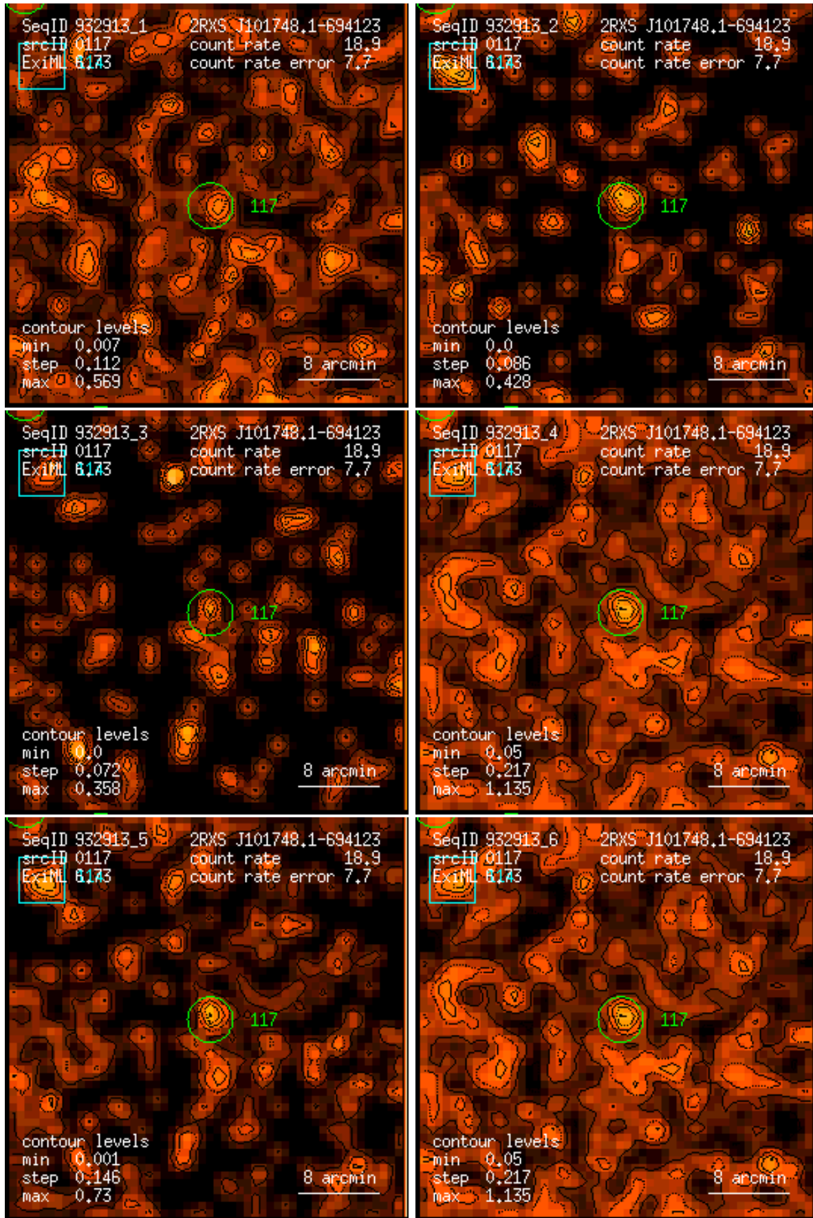
Figure 117: RASS 932913: detection 0117: band rate images, Gaussian filter: (1) PSPC channels 11 – 41, (2) 52 – 90, (3) 91 – 201, (4) 11 – 235, (5) 52 – 201, (6) 11 – 201. Broad band rates in counts/ks. Band rate contour levels in counts/ks/arcmin 2 .
