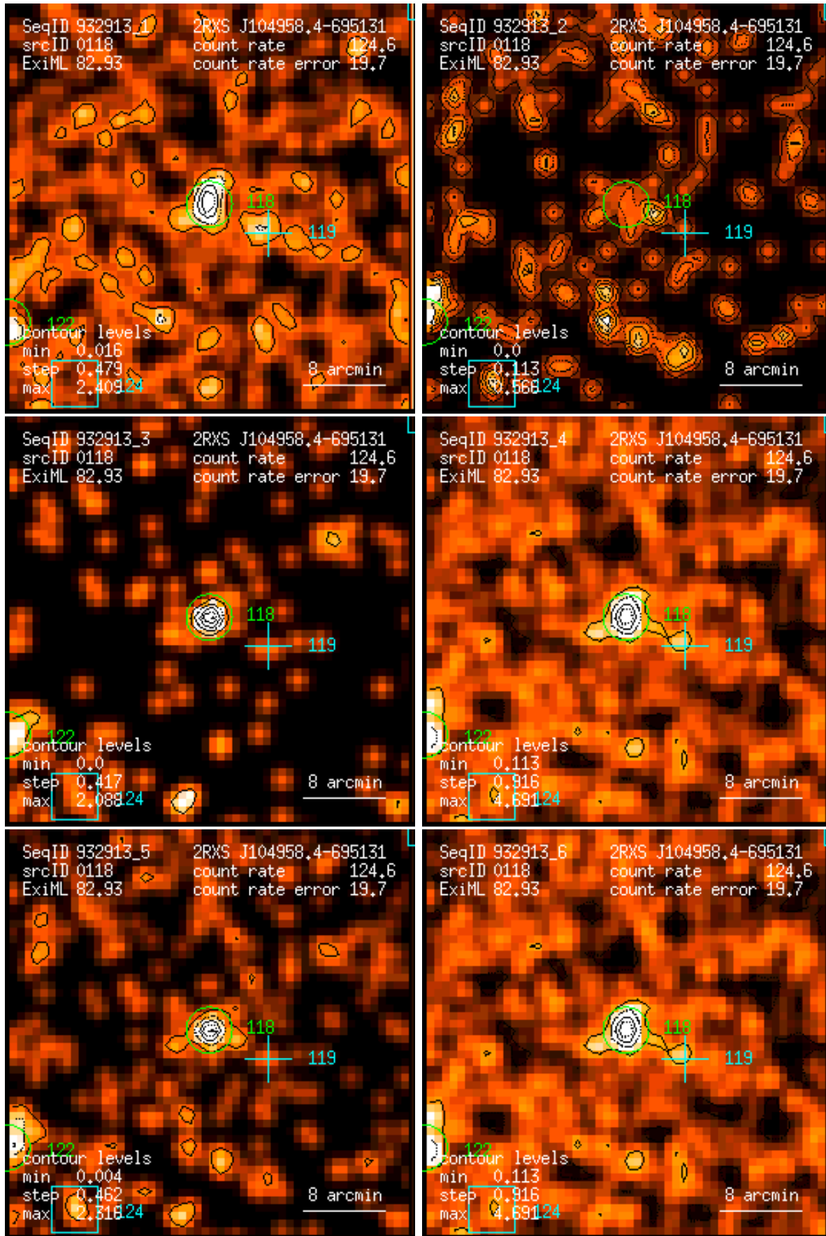
Figure 118: RASS 932913: detection 0118: band rate images, Gaussian filter: (1) PSPC channels 11 – 41, (2) 52 – 90, (3) 91 – 201, (4) 11 – 235, (5) 52 – 201, (6) 11 – 201. Broad band rates in counts/ks. Band rate contour levels in counts/ks/arcmin 2 .
