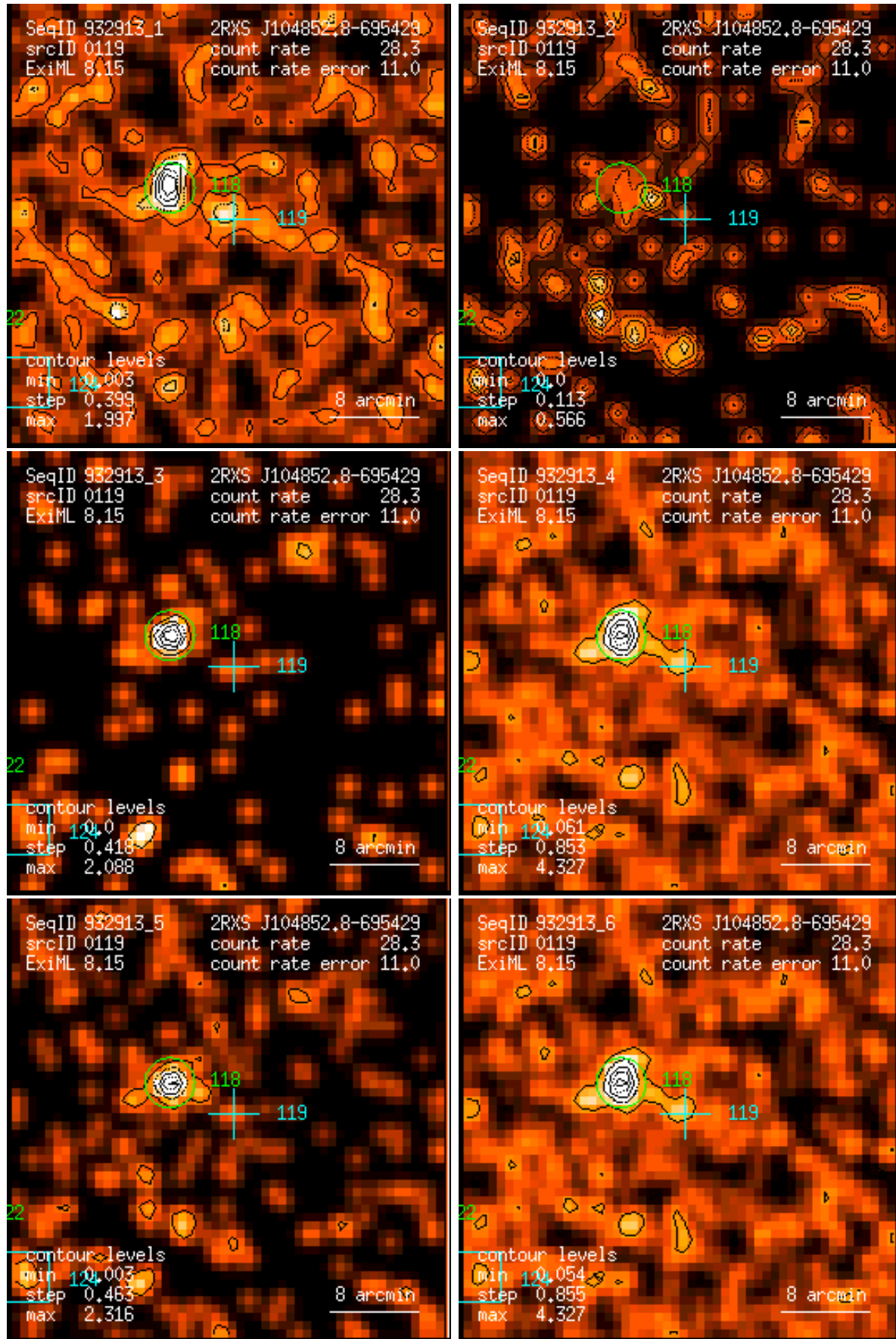
Figure 119: RASS 932913: detection 0119: band rate images, Gaussian filter: (1) PSPC channels 11 – 41, (2) 52 – 90, (3) 91 – 201, (4) 11 – 235, (5) 52 – 201, (6) 11 – 201. Broad band rates in counts/ks. Band rate contour levels in counts/ks/arcmin 2 .
