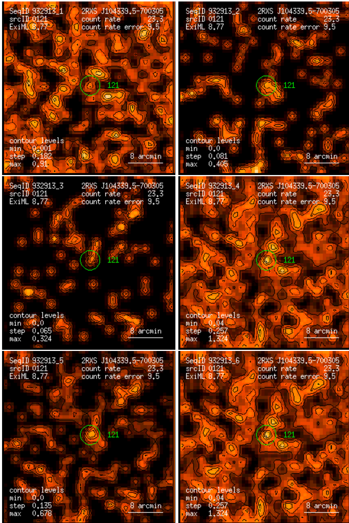
Figure 121: RASS 932913: detection 0121: band rate images, Gaussian filter: (1) PSPC channels 11 – 41, (2) 52 – 90, (3) 91 – 201, (4) 11 – 235, (5) 52 – 201, (6) 11 – 201. Broad band rates in counts/ks. Band rate contour levels in counts/ks/arcmin 2 .
