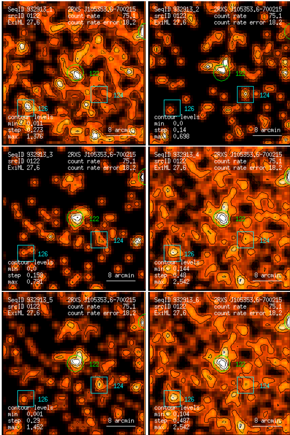
Figure 122: RASS 932913: detection 0122: band rate images, Gaussian filter: (1) PSPC channels 11 – 41, (2) 52 – 90, (3) 91 – 201, (4) 11 – 235, (5) 52 – 201, (6) 11 – 201. Broad band rates in counts/ks. Band rate contour levels in counts/ks/arcmin 2 .
