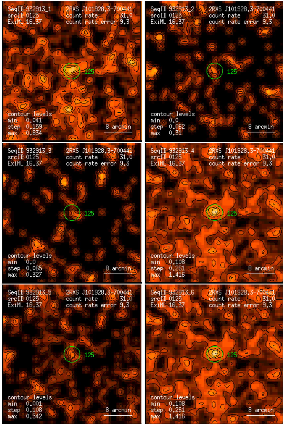
Figure 125: RASS 932913: detection 0125: band rate images, Gaussian filter: (1) PSPC channels 11 – 41, (2) 52 – 90, (3) 91 – 201, (4) 11 – 235, (5) 52 – 201, (6) 11 – 201. Broad band rates in counts/ks. Band rate contour levels in counts/ks/arcmin 2 .
