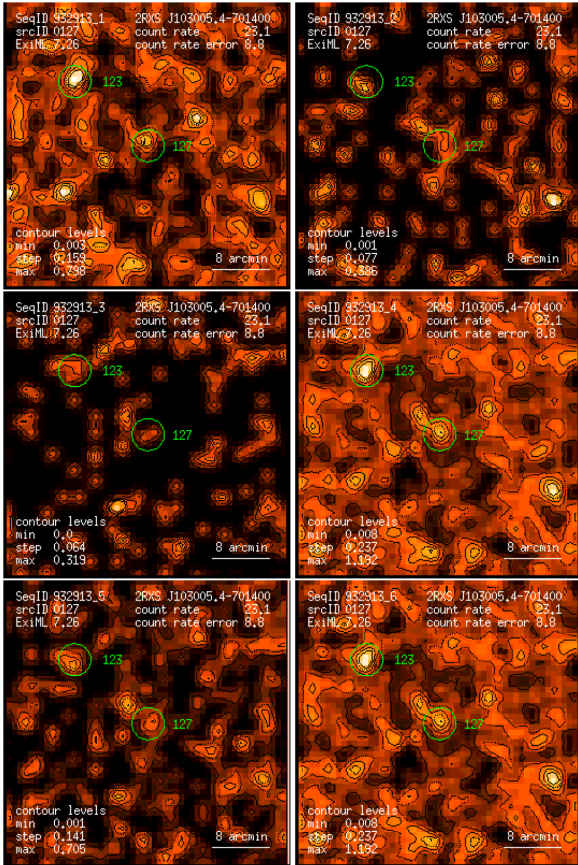
Figure 127: RASS 932913: detection 0127: band rate images, Gaussian filter: (1) PSPC channels 11 – 41, (2) 52 – 90, (3) 91 – 201, (4) 11 – 235, (5) 52 – 201, (6) 11 – 201. Broad band rates in counts/ks. Band rate contour levels in counts/ks/arcmin 2 .
