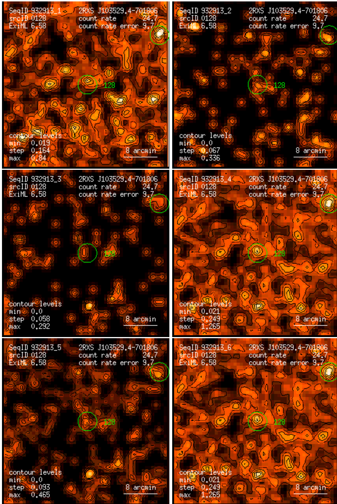
Figure 128: RASS 932913: detection 0128: band rate images, Gaussian filter: (1) PSPC channels 11 – 41, (2) 52 – 90, (3) 91 – 201, (4) 11 – 235, (5) 52 – 201, (6) 11 – 201. Broad band rates in counts/ks. Band rate contour levels in counts/ks/arcmin 2 .
