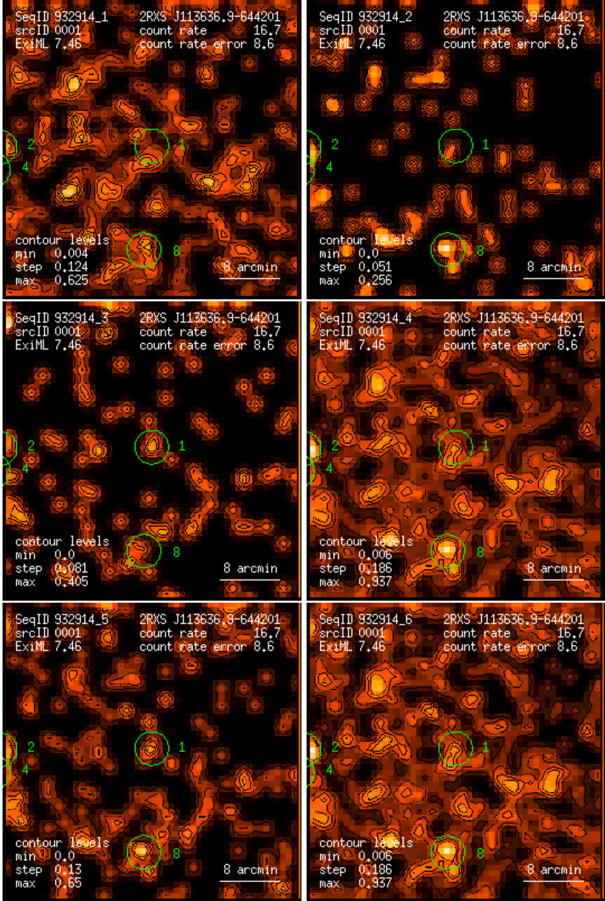
Figure 1: RASS 932914: detection 0001: band rate images, Gaussian filter: (1) PSPC channels 11 – 41, (2) 52 – 90, (3) 91 – 201, (4) 11 – 235, (5) 52 – 201, (6) 11 – 201. Broad band rates in counts/ks. Band rate contour levels in counts/ks/arcmin 2 .
