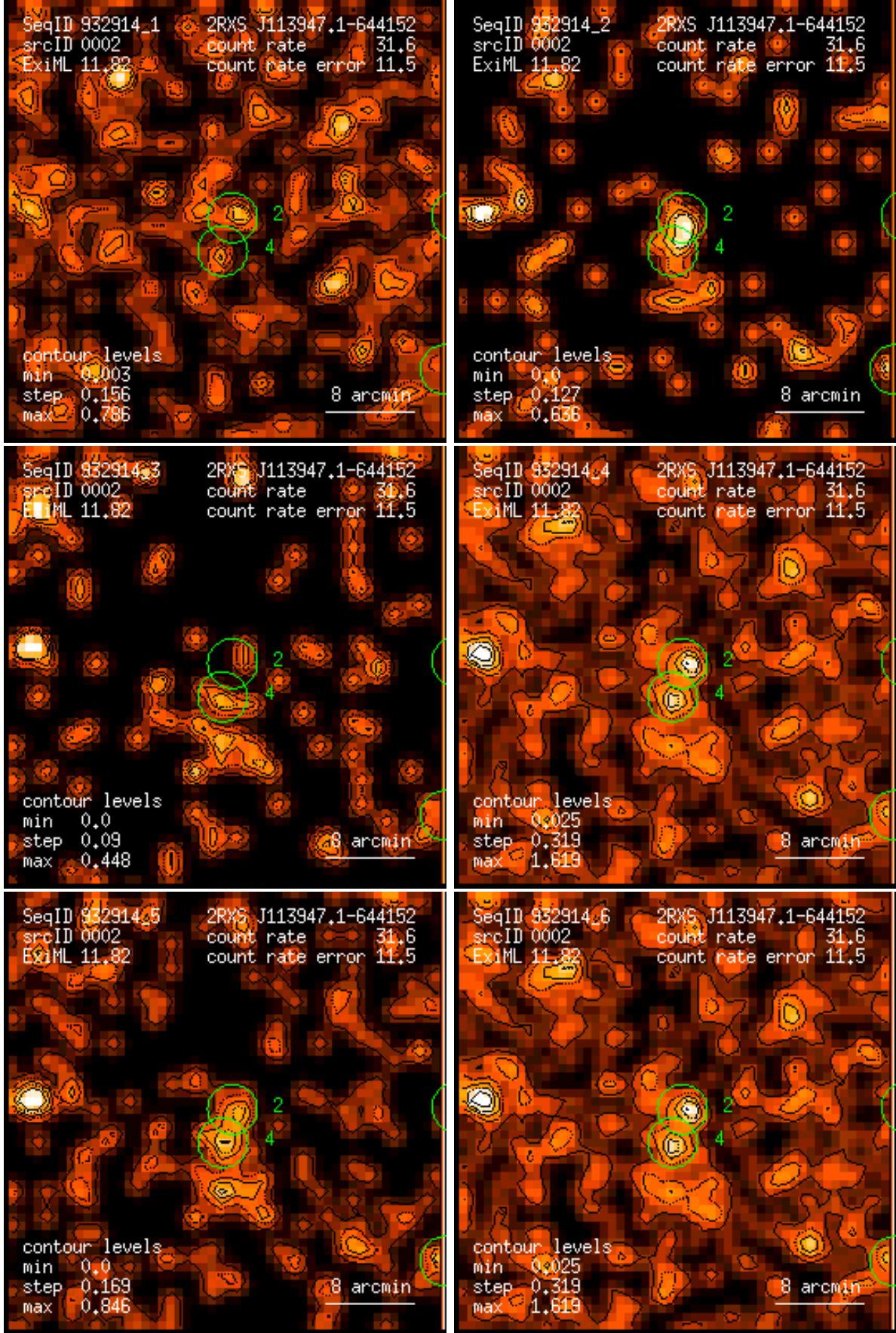
Figure 2: RASS 932914: detection 0002: band rate images, Gaussian filter: (1) PSPC channels 11 – 41, (2) 52 – 90, (3) 91 – 201, (4) 11 – 235, (5) 52 – 201, (6) 11 – 201. Broad band rates in counts/ks. Band rate contour levels in counts/ks/arcmin 2 .
