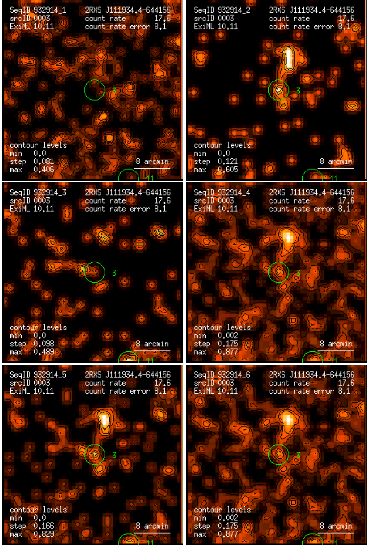
Figure 3: RASS 932914: detection 0003: band rate images, Gaussian filter: (1) PSPC channels 11 – 41, (2) 52 – 90, (3) 91 – 201, (4) 11 – 235, (5) 52 – 201, (6) 11 – 201. Broad band rates in counts/ks. Band rate contour levels in counts/ks/arcmin 2 .
