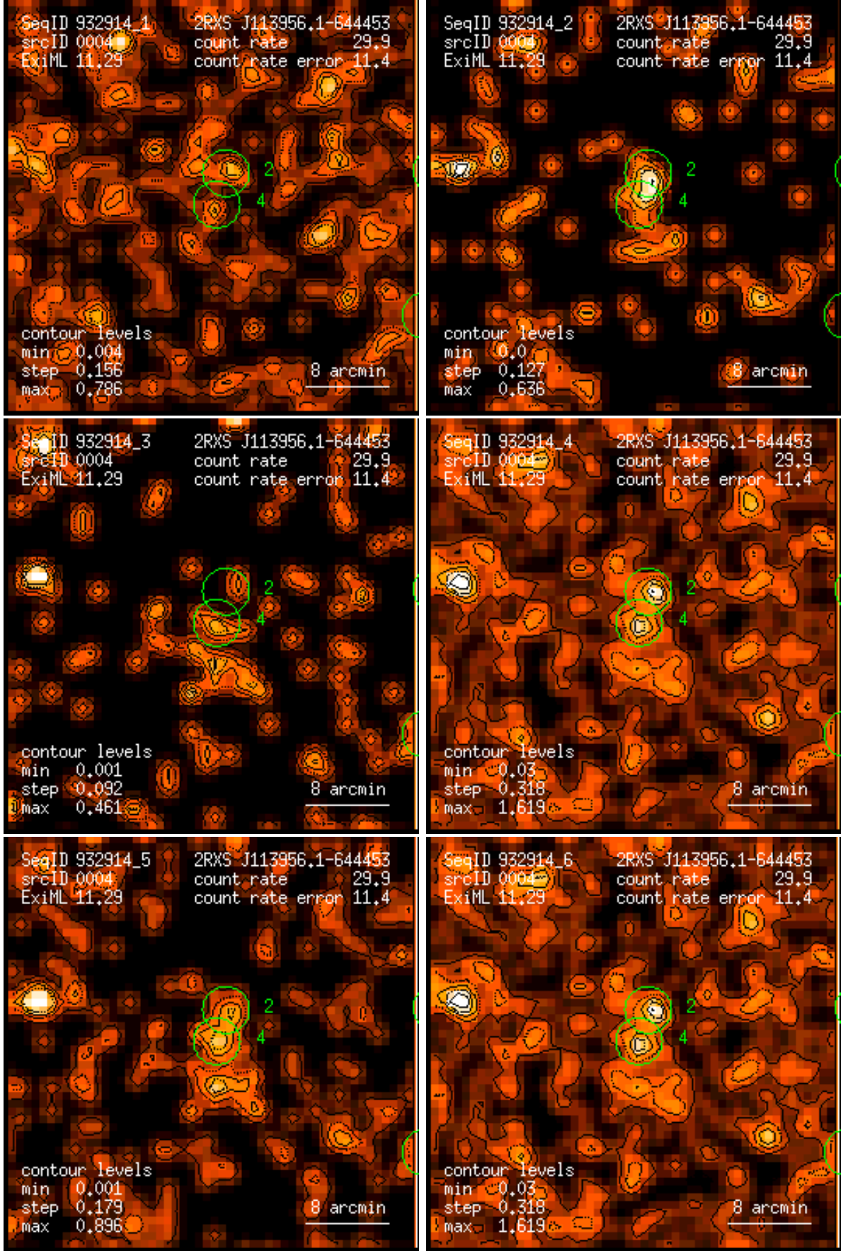
Figure 4: RASS 932914: detection 0004: band rate images, Gaussian filter: (1) PSPC channels 11 – 41, (2) 52 – 90, (3) 91 – 201, (4) 11 – 235, (5) 52 – 201, (6) 11 – 201. Broad band rates in counts/ks. Band rate contour levels in counts/ks/arcmin 2 .
