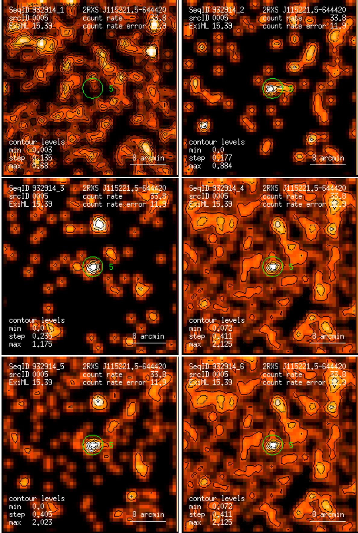
Figure 5: RASS 932914: detection 0005: band rate images, Gaussian filter: (1) PSPC channels 11 – 41, (2) 52 – 90, (3) 91 – 201, (4) 11 – 235, (5) 52 – 201, (6) 11 – 201. Broad band rates in counts/ks. Band rate contour levels in counts/ks/arcmin 2 .
