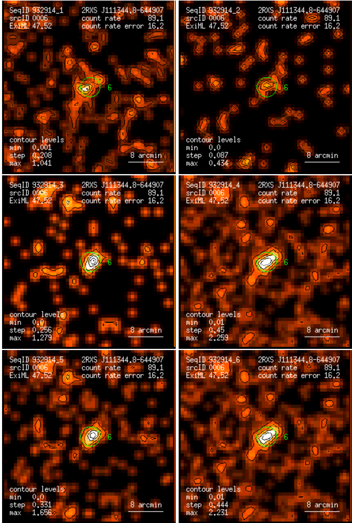
Figure 6: RASS 932914: detection 0006: band rate images, Gaussian filter: (1) PSPC channels 11 – 41, (2) 52 – 90, (3) 91 – 201, (4) 11 – 235, (5) 52 – 201, (6) 11 – 201. Broad band rates in counts/ks. Band rate contour levels in counts/ks/arcmin 2 .
