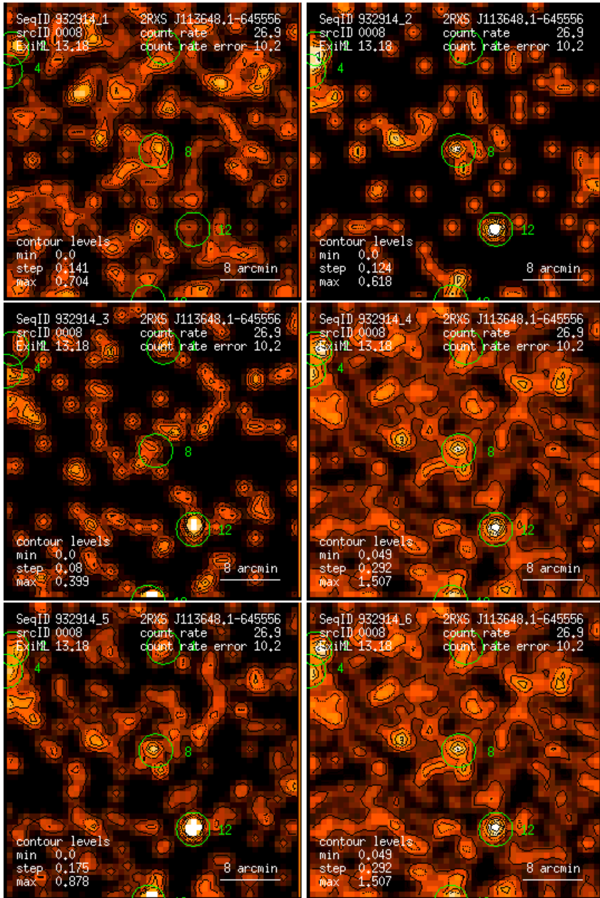
Figure 8: RASS 932914: detection 0008: band rate images, Gaussian filter: (1) PSPC channels 11 – 41, (2) 52 – 90, (3) 91 – 201, (4) 11 – 235, (5) 52 – 201, (6) 11 – 201. Broad band rates in counts/ks. Band rate contour levels in counts/ks/arcmin 2 .
