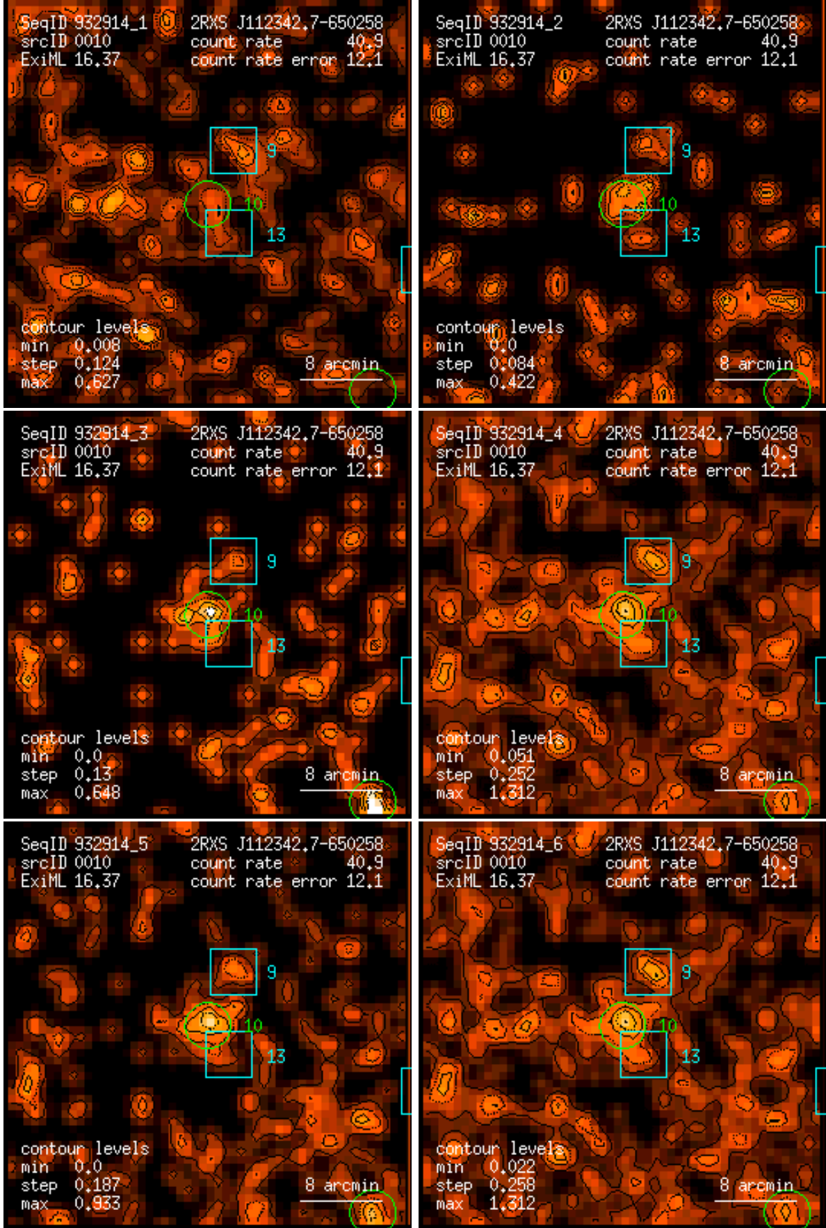
Figure 10: RASS 932914: detection 0010: band rate images, Gaussian filter: (1) PSPC channels 11 – 41, (2) 52 – 90, (3) 91 – 201, (4) 11 – 235, (5) 52 – 201, (6) 11 – 201. Broad band rates in counts/ks. Band rate contour levels in counts/ks/arcmin 2 .
