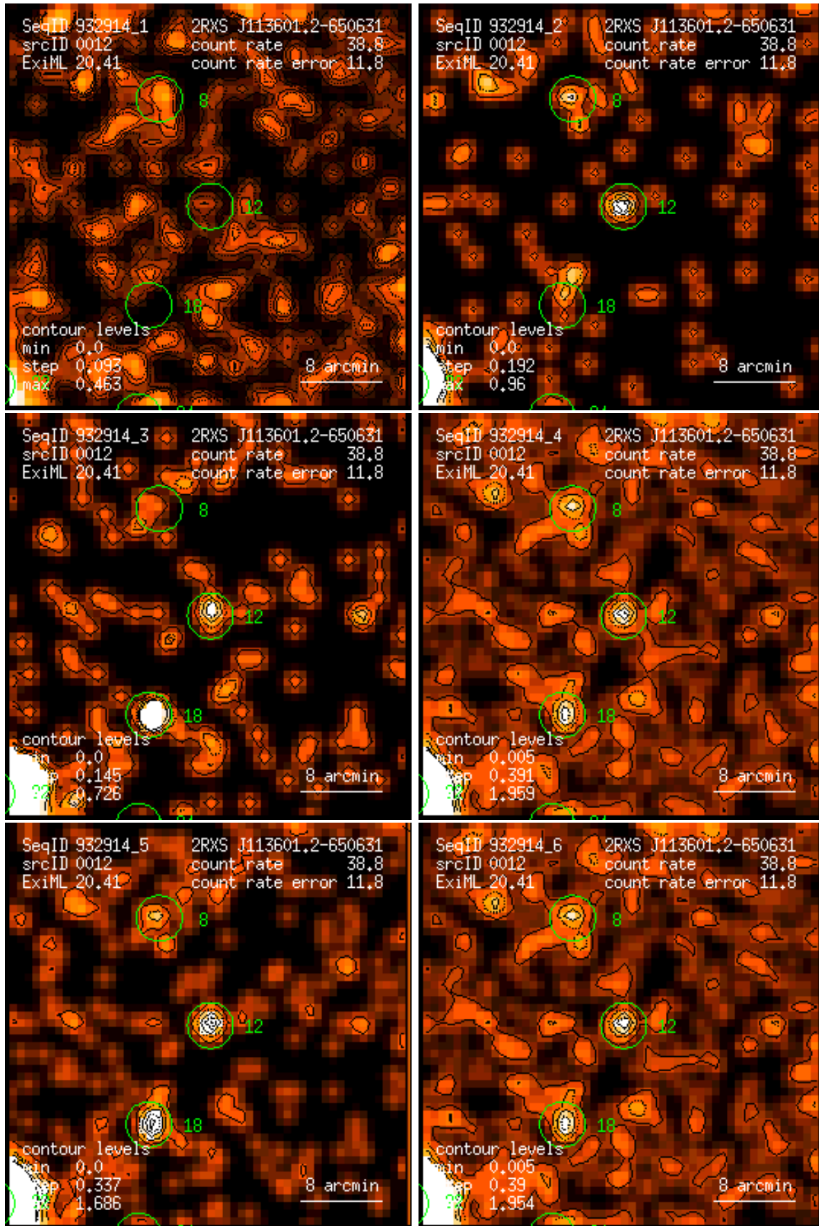
Figure 12: RASS 932914: detection 0012: band rate images, Gaussian filter: (1) PSPC channels 11 – 41, (2) 52 – 90, (3) 91 – 201, (4) 11 – 235, (5) 52 – 201, (6) 11 – 201. Broad band rates in counts/ks. Band rate contour levels in counts/ks/arcmin 2 .
