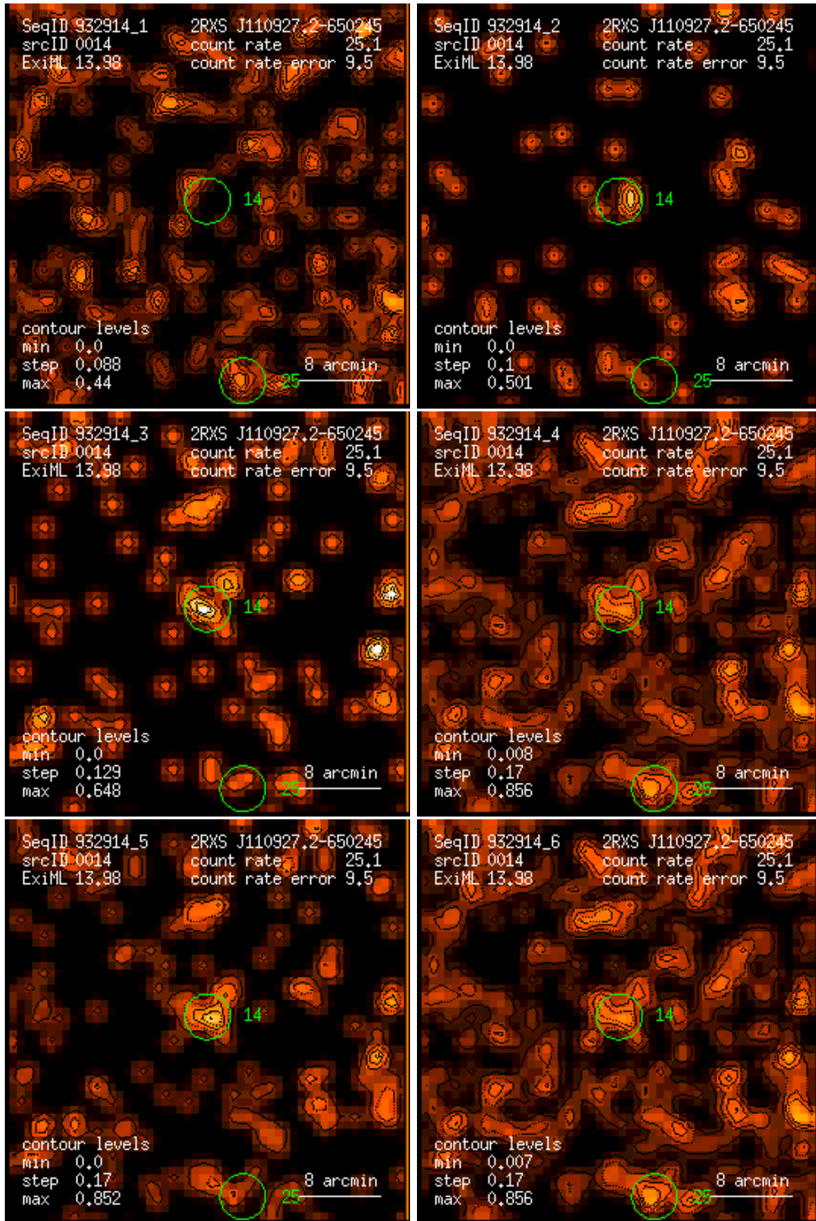
Figure 14: RASS 932914: detection 0014: band rate images, Gaussian filter: (1) PSPC channels 11 – 41, (2) 52 – 90, (3) 91 – 201, (4) 11 – 235, (5) 52 – 201, (6) 11 – 201. Broad band rates in counts/ks. Band rate contour levels in counts/ks/arcmin 2 .
