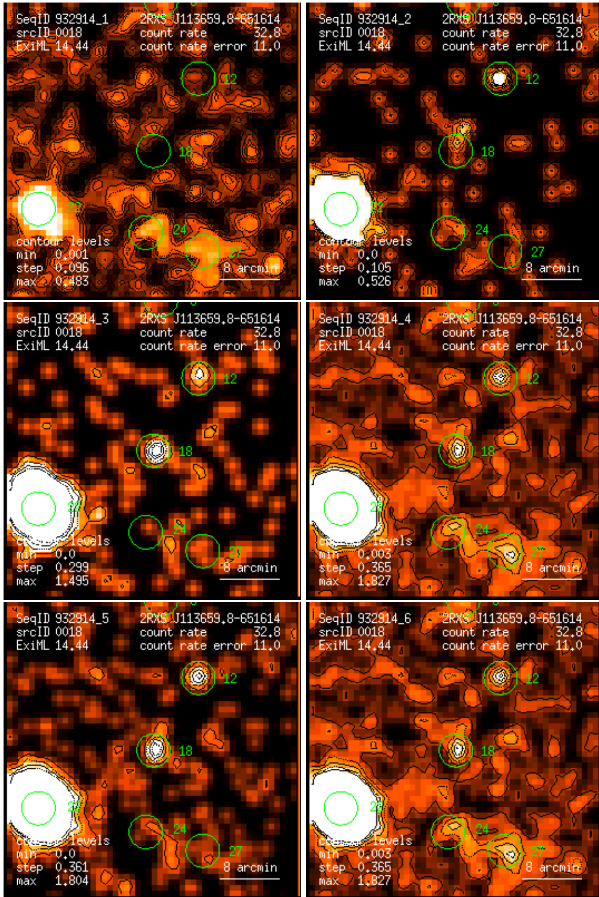
Figure 18: RASS 932914: detection 0018: band rate images, Gaussian filter: (1) PSPC channels 11 – 41, (2) 52 – 90, (3) 91 – 201, (4) 11 – 235, (5) 52 – 201, (6) 11 – 201. Broad band rates in counts/ks. Band rate contour levels in counts/ks/arcmin 2 .
