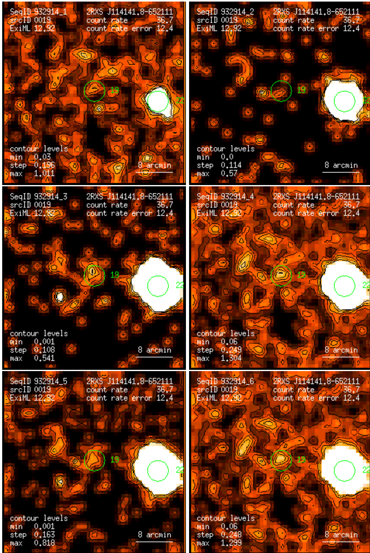
Figure 19: RASS 932914: detection 0019: band rate images, Gaussian filter: (1) PSPC channels 11 – 41, (2) 52 – 90, (3) 91 – 201, (4) 11 – 235, (5) 52 – 201, (6) 11 – 201. Broad band rates in counts/ks. Band rate contour levels in counts/ks/arcmin 2 .
