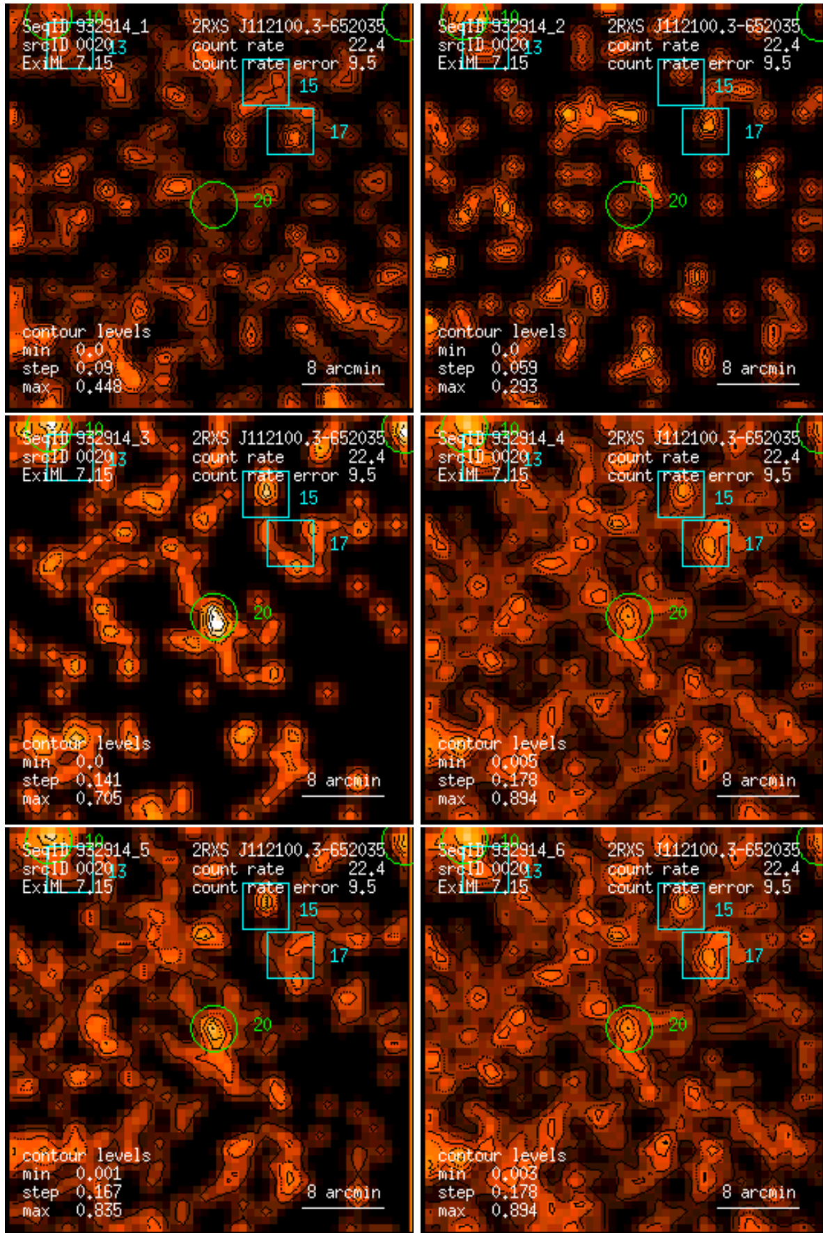
Figure 20: RASS 932914: detection 0020: band rate images, Gaussian filter: (1) PSPC channels 11 – 41, (2) 52 – 90, (3) 91 – 201, (4) 11 – 235, (5) 52 – 201, (6) 11 – 201. Broad band rates in counts/ks. Band rate contour levels in counts/ks/arcmin 2 .
