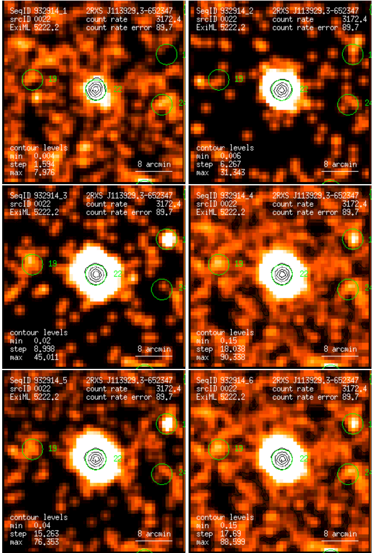
Figure 22: RASS 932914: detection 0022: band rate images, Gaussian filter: (1) PSPC channels 11 – 41, (2) 52 – 90, (3) 91 – 201, (4) 11 – 235, (5) 52 – 201, (6) 11 – 201. Broad band rates in counts/ks. Band rate contour levels in counts/ks/arcmin 2 .
