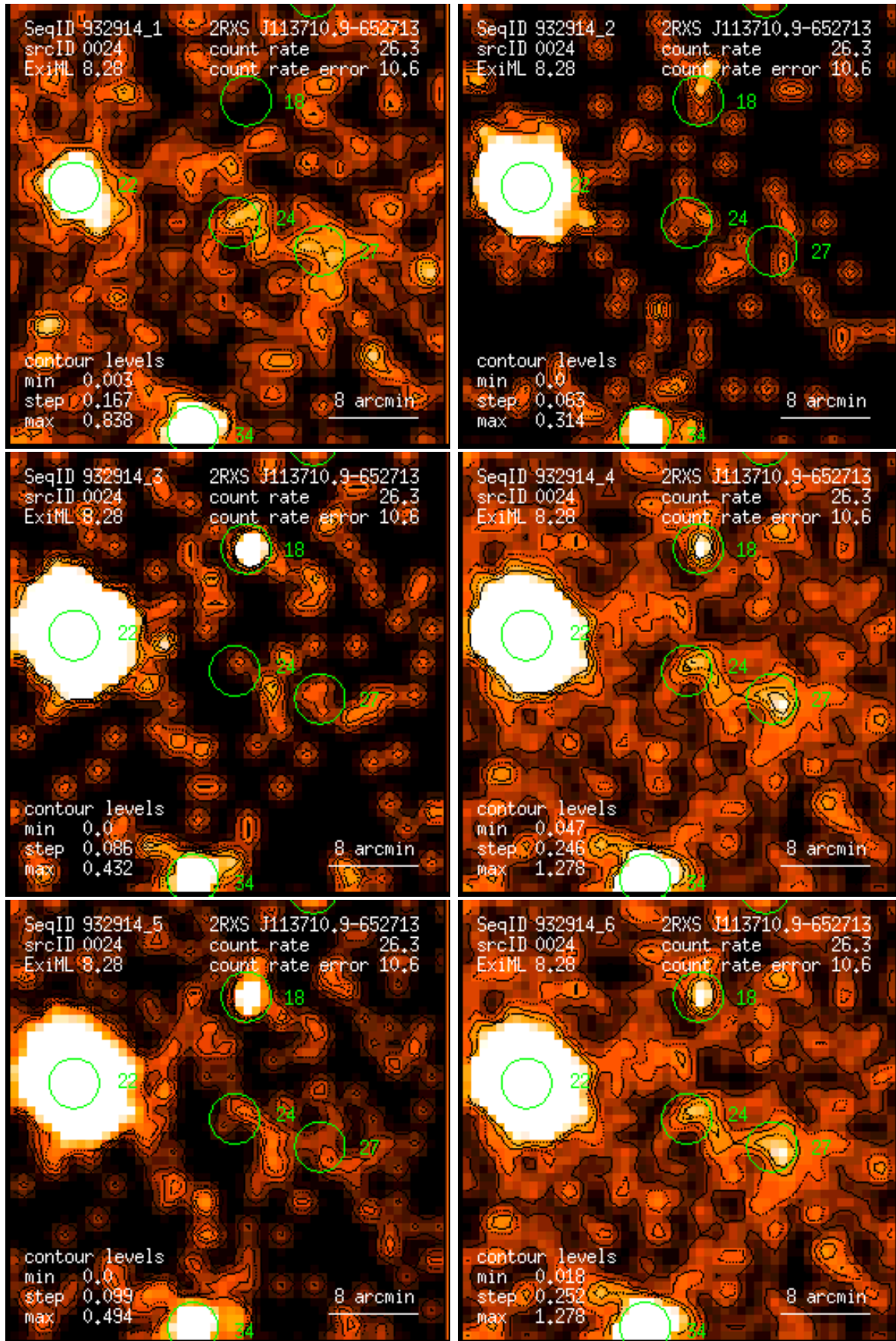
Figure 24: RASS 932914: detection 0024: band rate images, Gaussian filter: (1) PSPC channels 11 – 41, (2) 52 – 90, (3) 91 – 201, (4) 11 – 235, (5) 52 – 201, (6) 11 – 201. Broad band rates in counts/ks. Band rate contour levels in counts/ks/arcmin 2 .
