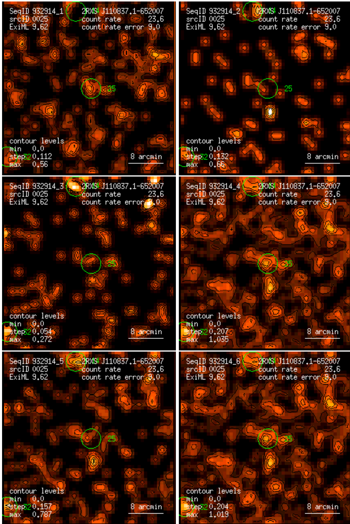
Figure 25: RASS 932914: detection 0025: band rate images, Gaussian filter: (1) PSPC channels 11 – 41, (2) 52 – 90, (3) 91 – 201, (4) 11 – 235, (5) 52 – 201, (6) 11 – 201. Broad band rates in counts/ks. Band rate contour levels in counts/ks/arcmin 2 .
