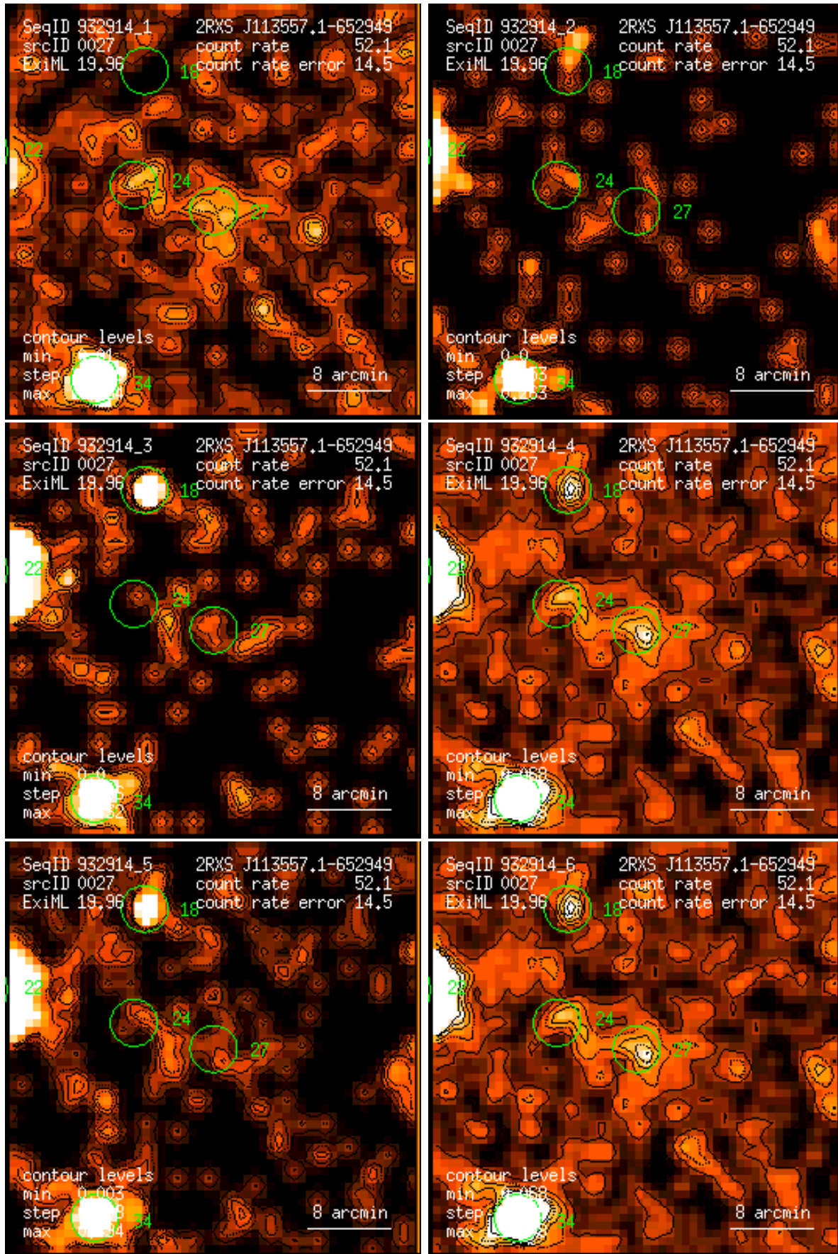
Figure 27: RASS 932914: detection 0027: band rate images, Gaussian filter: (1) PSPC channels 11 – 41, (2) 52 – 90, (3) 91 – 201, (4) 11 – 235, (5) 52 – 201, (6) 11 – 201. Broad band rates in counts/ks. Band rate contour levels in counts/ks/arcmin 2 .
